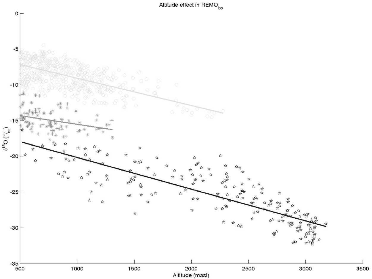
Figure 3.5: Variation of \delta^{18}\text{O} with altitude over the entire model domain, for the ECHAM-nested REMO simulation. Black pentagrams stand for Greenland, with a \delta^{18}\text{O} = -4.43 \cdot 10^{-3} \cdot h - 15.8 \text{‰} and a R^2 = 0.691 . Dark grey stars stand for the Scandinavian mountain range, with a \delta^{18}\text{O} = -2.39 \cdot 10^{-3} \cdot h - 13.1 \text{‰} and a R^2 = 0.116 . Light grey circles stand for central Europe massifs, with a \delta^{18}\text{O} = -3.82 \cdot 10^{-3} \cdot h - 5.27 \text{‰} and a R^2 = 0.421 .
