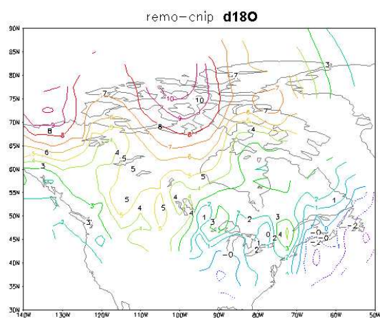
Figure B.3: Difference in mean annual \delta^{18}\text{O} between \text{REMO}_{iso} and CNIP data set. Values taken at the location of the CNIP stations are subtracted to each other, and the resulting field is interpolated to underline the spatial patterns of REMO discrepancies.
