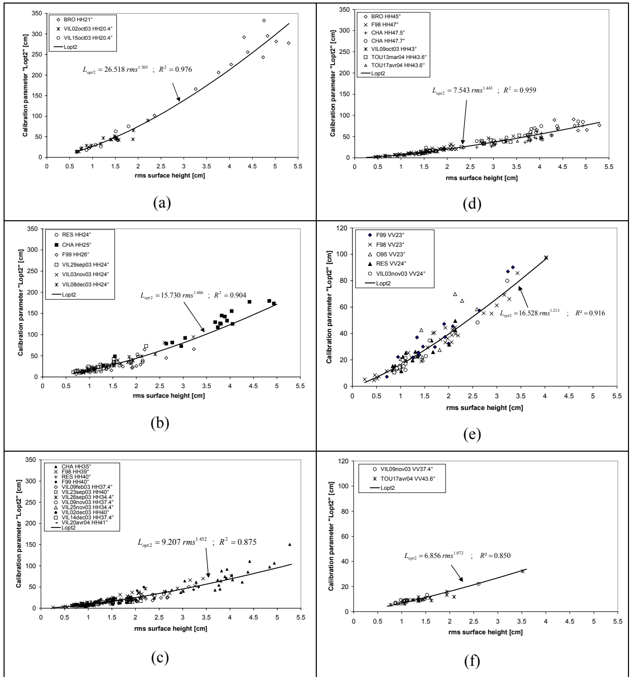
Figure 4. The calibration parameter Lopt2 as a function of surface height for radar configurations in C-band, HH and VV polarizations, and incidence angles between 20° and 48°. The ASAR database (VILxxx and TOUxxx) was used to supplement the database employed by Baghdadi et al. (2004).
