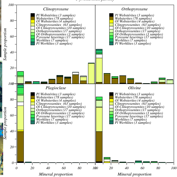
Fig. 10 Pyroxenites family
