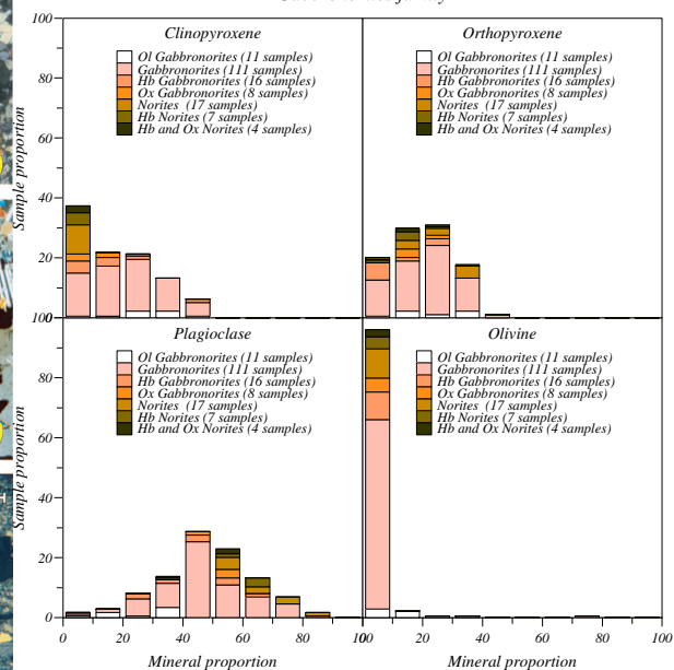
Fig. 8 Gabbronorites family
