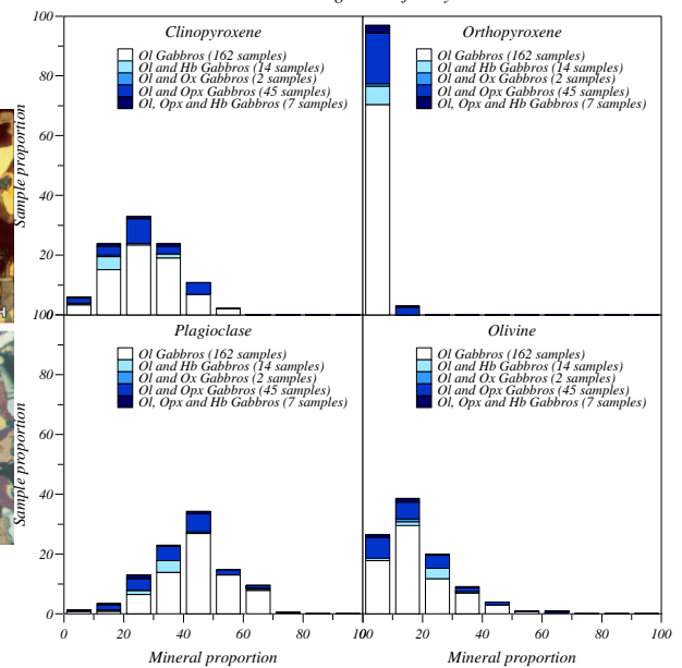
Fig. 6 Olivine gabbros family
