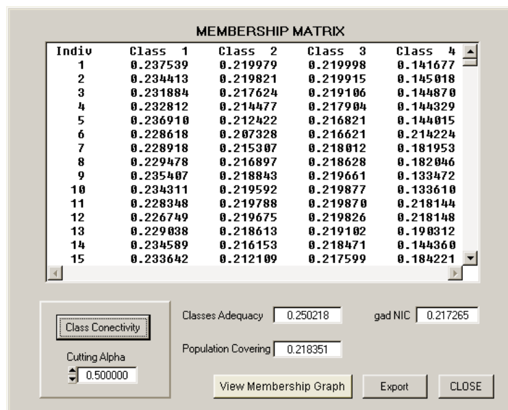
Figure 25 - Analyse Window
