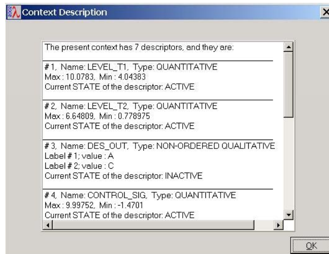
Figure 15 – Context Description window
