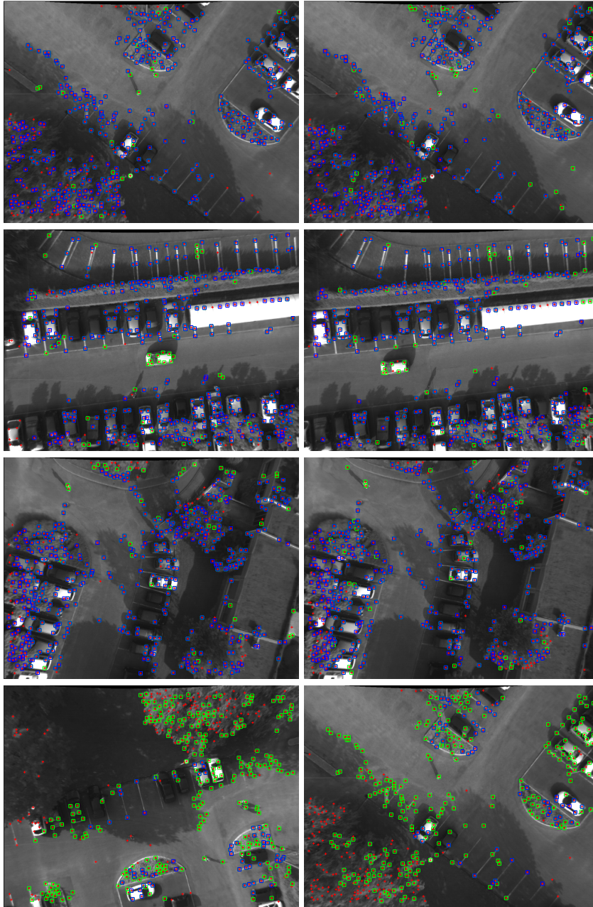
Figure 4.7: Interest points matched between some consecutive images of the sequence of the trajectory shown in figure 4.6 - the blue squares are the matched point. Each line shows two consecutive images, except the last one that shows the matches established between the image number 390 at the end of the trajectory and the first image (landmark re-perception).
