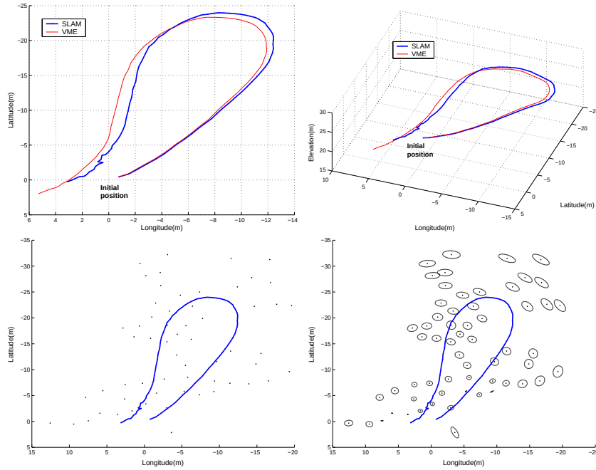
Figure 4.2: A first result of our SLAM implementation with a sequence of 90 stereovision pair, taken at altitudes ranging from 20 to 25 m . Top image show the reconstructed trajectory in orthogonal projection and in 3D. Bottom images show the 60 landmarks mapped, with 1\sigma uncertainty ellipses (left: real scale, right: magnified by a factor of 40)
