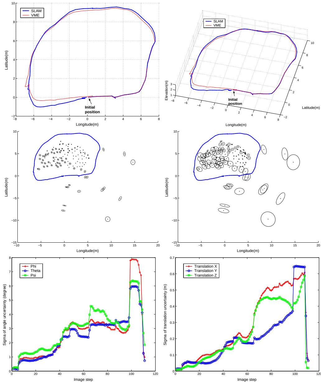
Figure 4.8: A result of our SLAM implementation with Lama, with a sequence of 110 stereovision pairs. Top images show the reconstructed robot trajectory in orthogonal projection and in 3D. Middle images show the 118 landmarks mapped, with 1\sigma uncertainty ellipses (left: real scale, right: magnified by a factor of 5), and bottom images show the evolution of the standard deviations of the robot position parameters.
