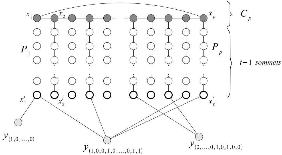
FIG. 4.5 – Construction de \mathcal{G}(\mathcal{C}_p) .
