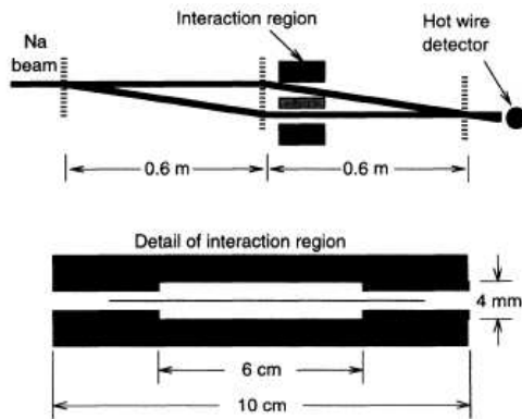
FIG. 1. Schematic of our interferometer and interaction region. Vertical dashed lines are 200-nm-period diffraction gratings. The detail of the interaction region shows the 10- \mu m copper foil suspended between the side plates. The guard electrodes are indicated in black at both ends.
