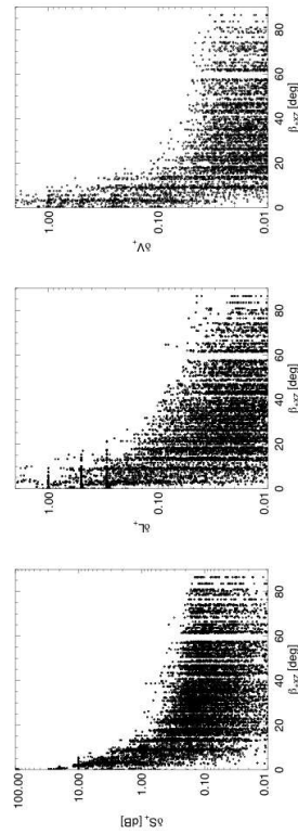
FIGURE 8: \delta S_+ , \delta L_+ and \delta V_+ vs. \beta_{+XZ} in case of RPWS-like digitization errors.
