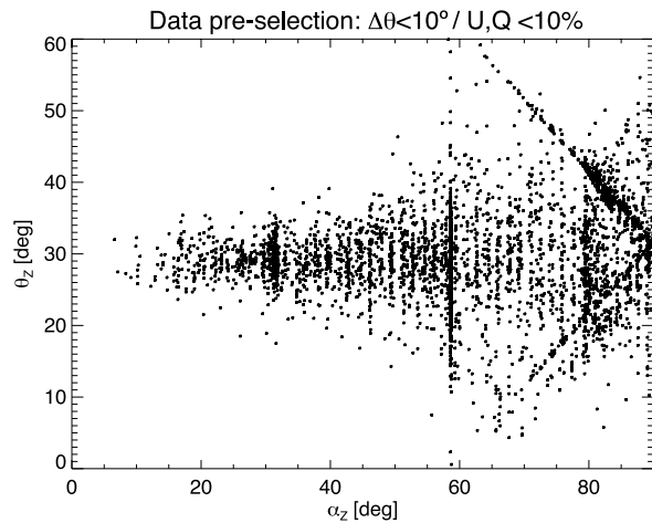
Figure 14. RPWS Calibration data at Jupiter: resulting Z antenna colatitude ( \theta_Z ) versus \alpha_Z . The data preselection applied to the data is the following: the angular distance from the wave direction of arrival to the position of Jupiter is < 10^\circ ; the degree of linear polarizations U ; and Q are < 10\% . These wave parameters come from a preliminary DF inversion run on the data. The shape of the cloud of points is very similar to the one simulated for a 10% residual linear polarization (see Figure 13e). Thick vertical lines (at \alpha_Z \sim 30^\circ and \alpha_Z \sim 60^\circ ) corresponds to unwanted emissions still selected by our data preselection (e.g., solar type 3 bursts, that have no polarization and comes from the Sun direction, opposite to the Jupiter direction).
