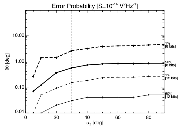
Figure 12. Error probability levels on the source position \delta\theta caused by the digitization for the circular polarization DF inversion. The errors probability levels are displayed for different \alpha_Z^{\text{lim}} and 8-bit/12-bit digitization.
