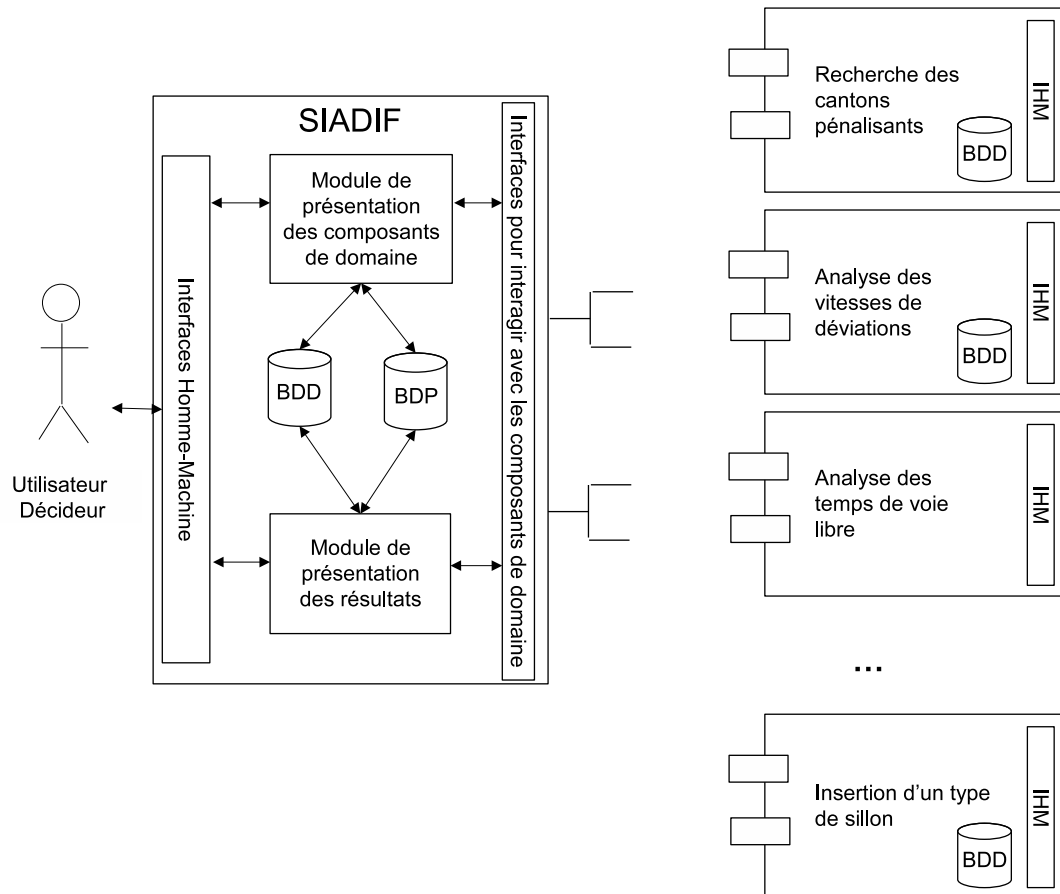
FIGURE 4.30 – Architecture de SIADIF
