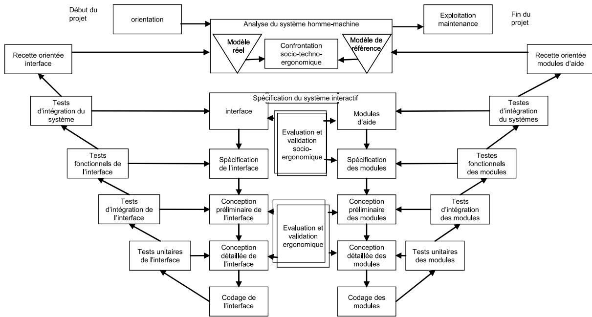
FIGURE 2.9 – Modèle ∇ [Kolski, 1995, Kolski, 1997]
