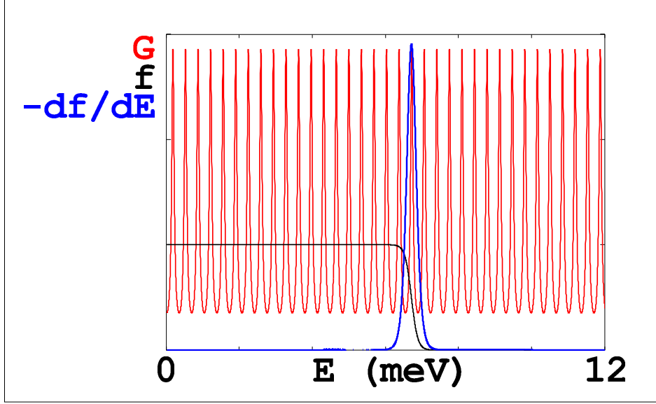
Figure 1.6: Schematic presentation of DOS modulation (red), Fermi distribution function and its derivative. Parameters for the calculation are as follows: B = 0.2T , \Gamma = 0.05\text{meV} , E_f = 6.7\text{meV} , T = 1K
