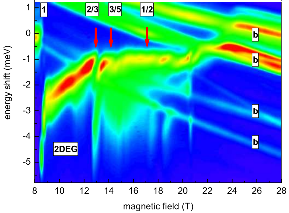
Figure 5.7: Intensity map of the photoluminescence of the NTT-C sample at T=30\text{mK} .
