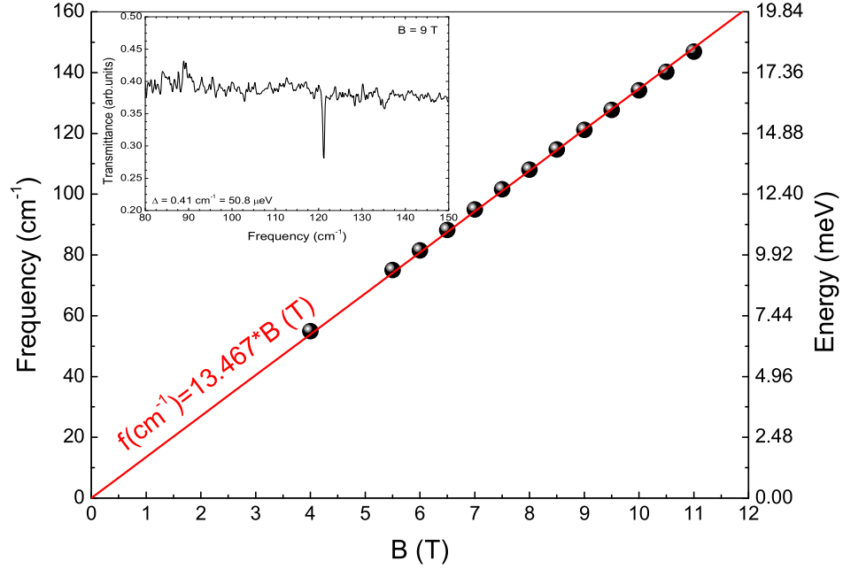
Figure 4.6: Determination of the electron effective mass from cyclotron resonance measurements. Inset. Normalised transmission spectrum at B=9\text{T} of the NTT-A sample. Data from [3].
