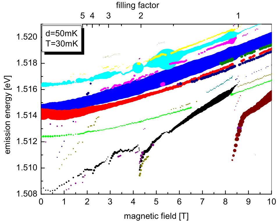
Figure 4.16: Complex PL spectra with all 2DEG and bulk lines. Emission energy versus magnetic field. Circle diameter corresponds to line intensity.
