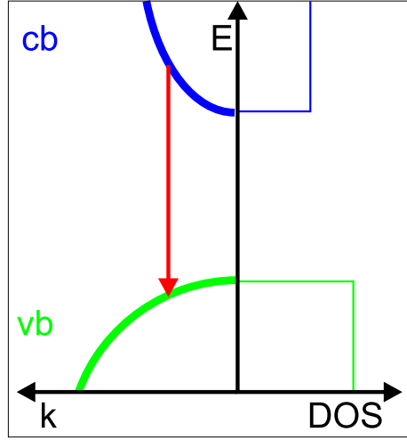
Figure 4.7: Energy dispersion, density of states and a recombination process schematically presented for a quantum well.
