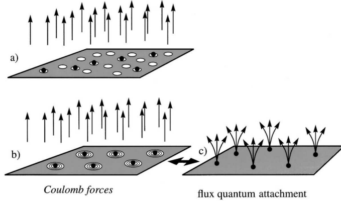
Figure 1.13: Schematic picture for the \nu = 1/3 fractional quantum Hall state. Electrons marked as dots, vortices as discs, magnetic flux quanta as arrows. a) One vortex on each electron with 2/3 of vortices unattached. b) The e-e repulsion is reduced by placing additional vortices on the electrons. c) Situation b) viewed as composite particles made from electrons and the attached flux quanta. Picture from [20].
