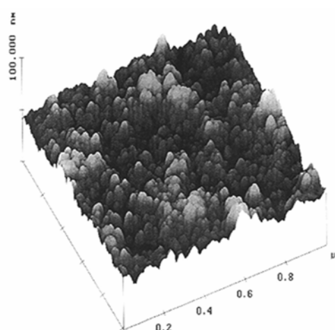
SnO 2 + 10% Pd (Rms = 6,7 nm)
