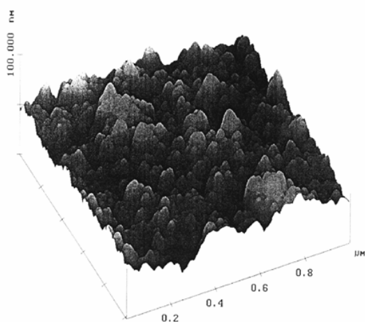
SnO 2 + 3%Pd (Rms = 6,4 nm)
