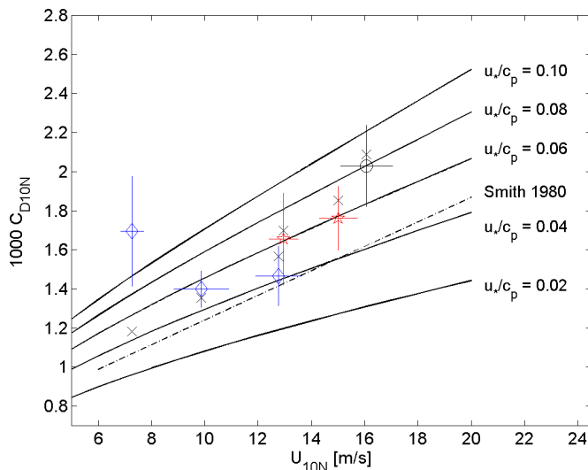
Figure 10: Drag coefficient versus wind speed, both 10m neutral, for FETCH wind sea data. The data are grouped by inverse wave age, 0.04 < u_* / c_p \leq 0.06 ( \diamond ), 0.06 < u_* / c_p \leq 0.08 ( \star ), and u_* / c_p > 0.08 ( \circ ), in wind speed bins of 3m/s, with the crosses indicating 1 standard deviation in C_{D10N} and U_{10N} . The \times 's represent the expected drag coefficient of each group based on its mean u_* / c_p and U_{10N} . The curves are Smith [1980], and the wave age dependent drag relations resulting from [5] and [9].
