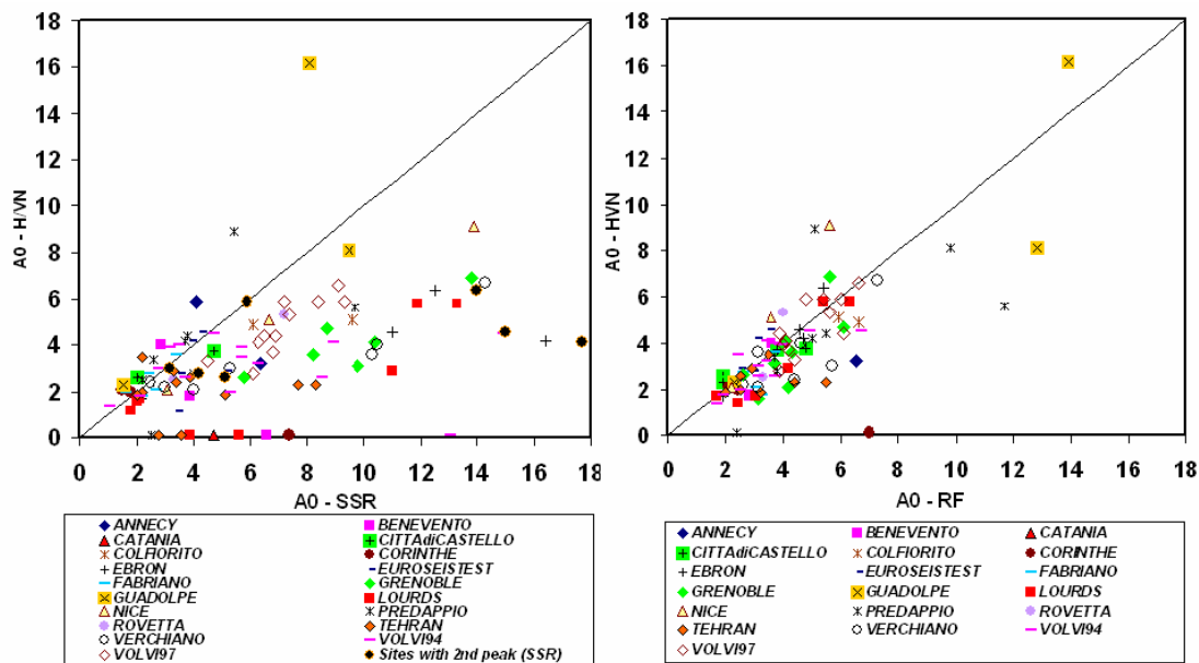
Figure 4.7 Correlation between H/V amplitude (A0-H/V noise) and SSR amplitude (A0-SSR) [left]; and RF amplitude (A0-H/V-Earthquake) [right]. The "symbols" on the x axis represent all the sites for which no A_{0HV} measurement could be performed because of the absence of any peak.
