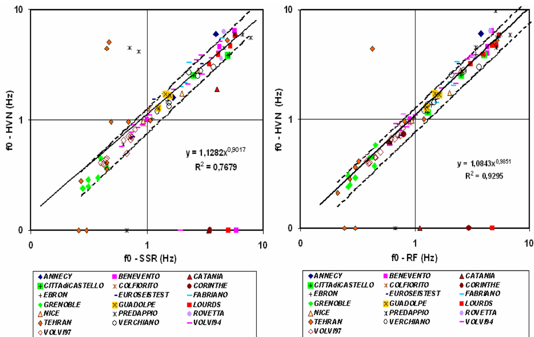
Figure 4.4: Correlation between H/V pick frequency (f0-H/V) and SSR fundamental frequency (f0-SSR) (left) and RF peak frequency (f0-H/V_earthquakes) (right) for the whole data set compiled within the SESAME project. The black line present the best fitting line and the dashed lines are the limits of \pm 25\% of f_{0SSR} . The "symbols" on the x axis represent all the sites for which no A_{0HV} measurement could be performed because of the absence of any peak.
