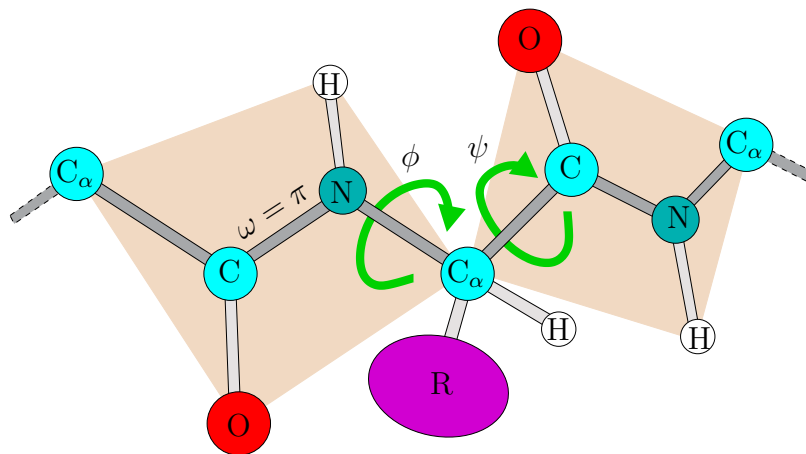
Figure 6.3: The elements in a protein are amino-acids connected via peptide bonds. Under the rigid geometry assumption, the peptide units are considered planar and only angles \phi and \psi are variable.
