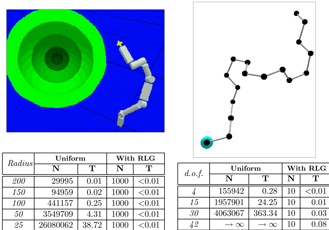
Figure 3.8: Two tests for analyzing the performance of RLG.
