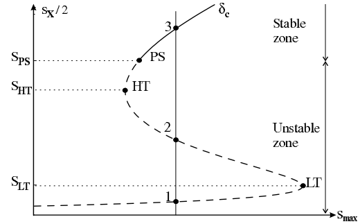
Figure 4. Bistability curve: linearly polarized field intensity S = s_x/2 as a function of s_{max} . PS is the switching threshold and HT and LT the higher and lower turning points. For certain incident intensities s_{max} three solutions (1, 2, 3) exist for the intracavity intensity s_x/2 , of which only one (3) is stable, instead of the usual two (1, 3) in the absence of the PS phenomenon.
