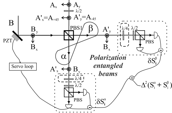
Figure 11. Polarization-entangled beam generation set-up. Using the quarter-wave plates or not allows for measuring either S_{S_2} or S_{S_3} .
