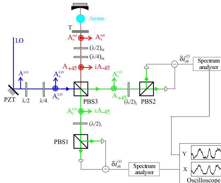
Figure 4. Experimental set-up.
