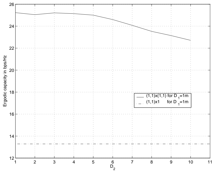
FIG. 5.27 – Capacity behavior in the surrounding region of the two transmitters.
