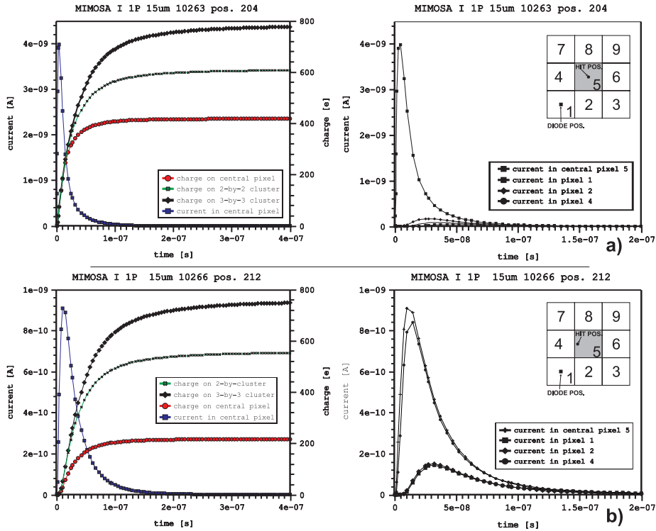
Figure 4-6: Transient simulation results for the single-diode pixel configuration with a 15\ \mu\text{m} epitaxial layer thick. Collected charge and selected contact currents for the (a) central and (b) the side particle impact.
