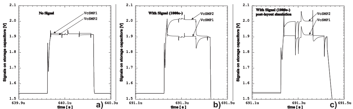
Figure 7-9: Simulated response of the pixel amplifier, measured as a voltage on two store capacitors, (a) in the case of absence of any charge deposited, (b) and for signal equal 1000 e^- schematic only, and (c) post-layout simulation.
