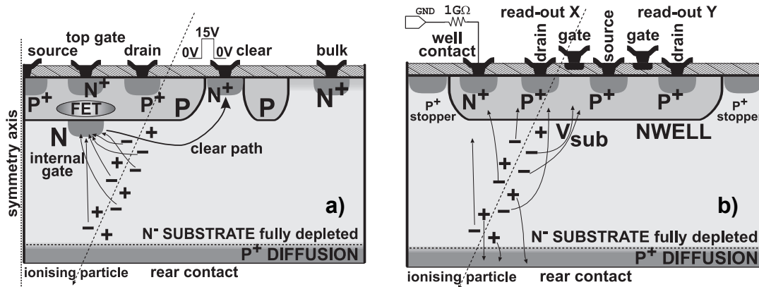
Figure 3-14: (a) Working principle of the DEPFET detector and (b) the pMOS pixel detector.
