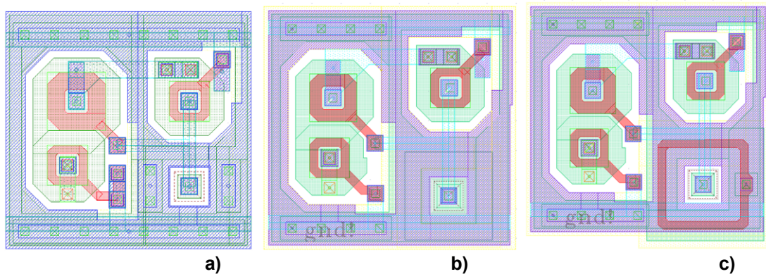
Figure C-8: Example of basic cell layout in MIMOSA III: (a) single-diode pixel with enclosed transistors (1P_EN), (b) single-diode pixel with enclosed transistors and STI region removed in the vicinity of the diode (1P_RH_EN), (c) single-diode pixel with enclosed transistors and polysilicon grounded ring around diode (1P_EN_NPOL_GND). The last metal level (M3) is not shown.
