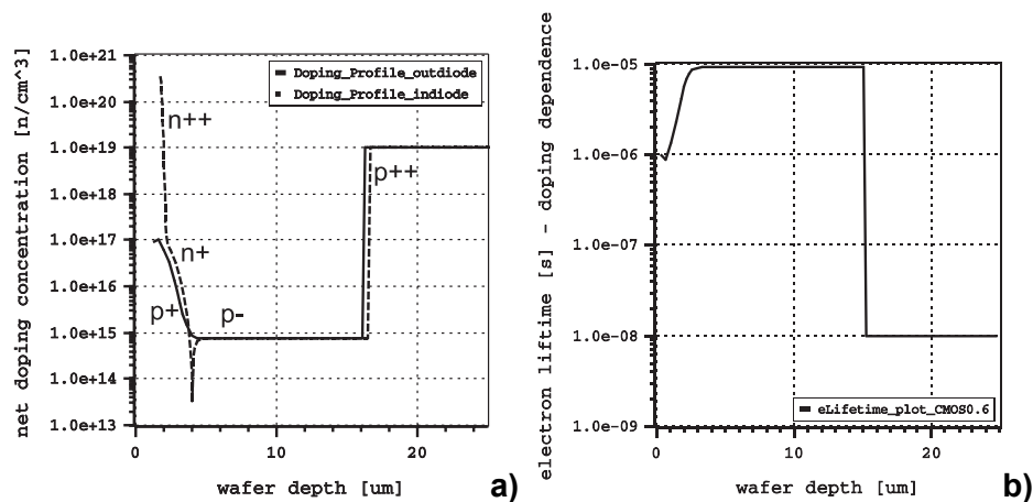
Figure 4-1: (a) Doping profiles, used in the detector simulations, as a function of the wafer depth, (b) electron lifetime profile resulting from doping dependence.
