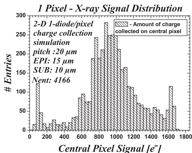
Figure 5-12: Pulse height distribution obtained in two-dimensional simulation of charge collection in one diode configuration of pixel pitch of 20\ \mu\text{m} and an epitaxial layer thickness of 15\ \mu\text{m} .
