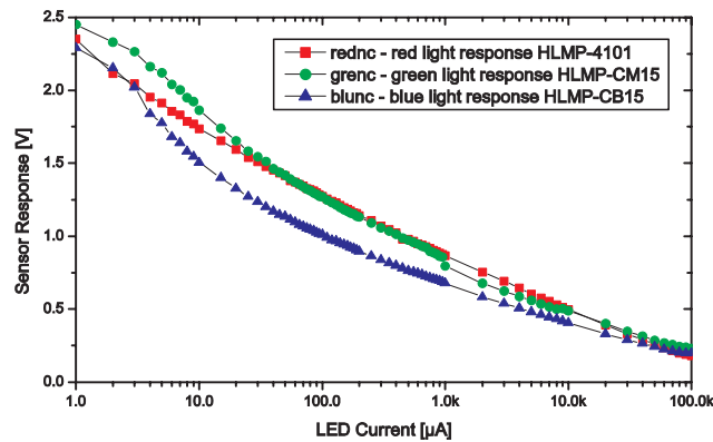
Figure 7-6: Response of the two-diode logarithmic pixel to LED diode sources of different wavelengths RGB (626 nm, 524 nm, 470 nm).
