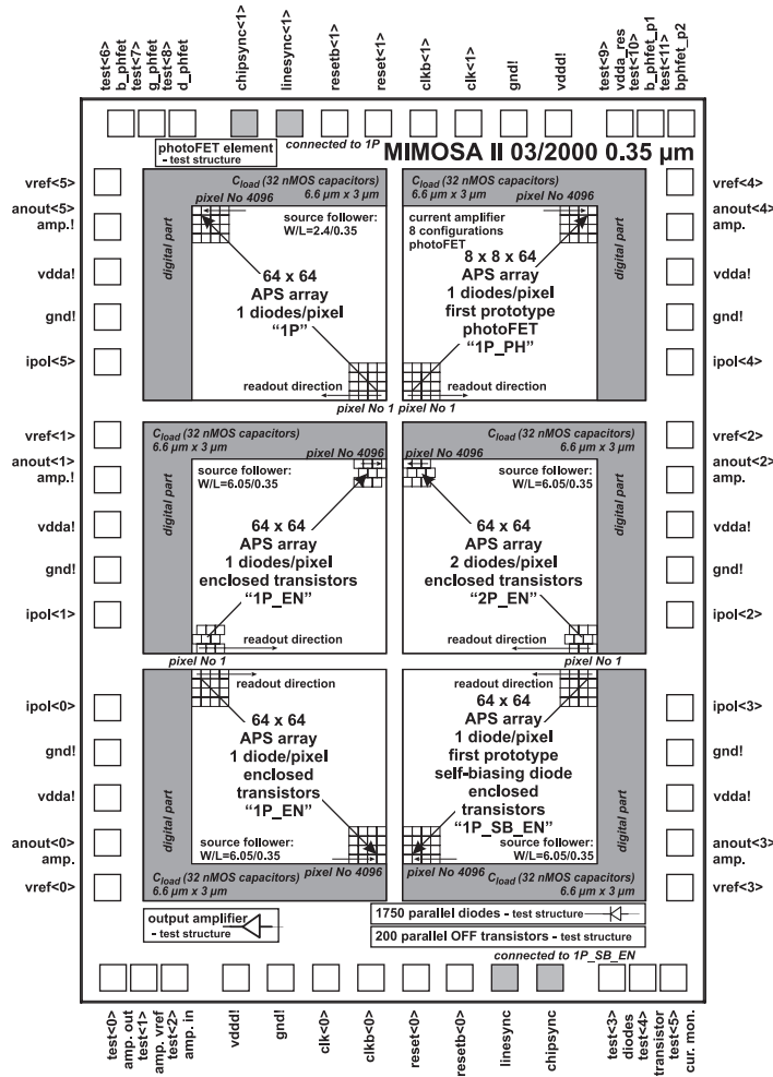
Figure C-5: Simplified structure and pin-out of the MIMOSA II chip (Alcatel Mietec 0.35 \mu\text{m} ).
