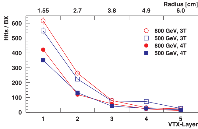
Figure 1-7: Number of hits resulting from pair background in the five layers of vertex detector for a magnetic field of 3 T and 4 T and for \sqrt{s} of 500 GeV and 800 GeV (from TESLA TDR)
