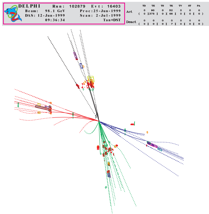
Figure 1-6: Four-jet event \bar{b}bq\bar{q} at 200 GeV taken at the DELPHI experiment considered as a candidate for Higgs boson discovery (from DELPHI collaboration).
