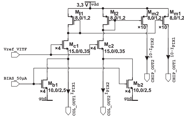
Figure 7-12: Column cascode termination circuitry.
