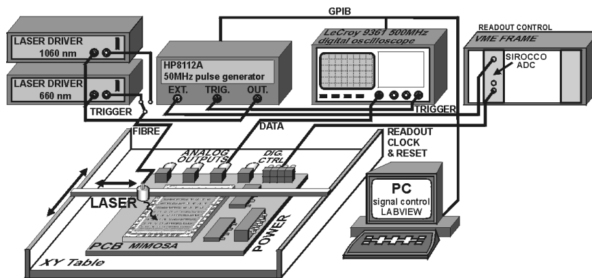
Figure 6-5: Set-up used for tests with infrared laser.
