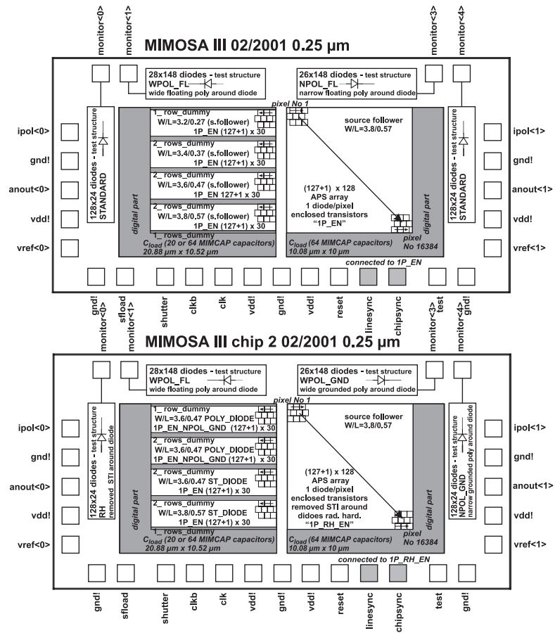
Figure C-7: Simplified structure and pin-out of the MIMOSA III chip (IBM 0.25 \mu\text{m} ).
