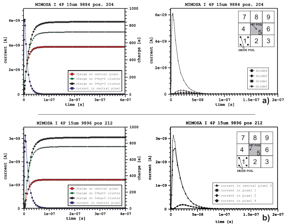
Figure 4-7: Transient simulation results for the four-diode pixel configuration with 15 \mu\text{m} epitaxial layer thick. Collected charge and selected contact currents for (a) the central and (b) the side particle impact.
