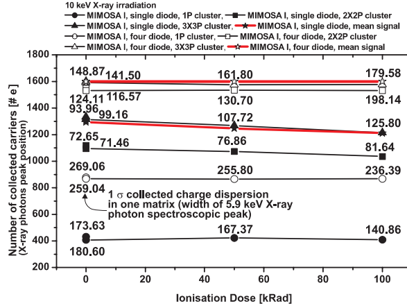
Figure 6-35: Number of collected charge carriers on the central pixel, 2 × 2 pixels and 3 × 3 pixels clusters for single and four diode pixel configurations in the MIMOSA I prototype.
