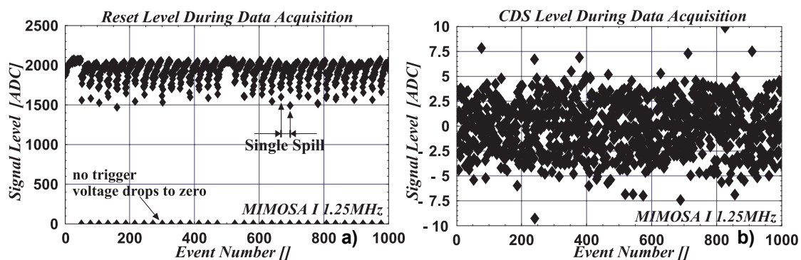
Figure 6-10: Effect of partial pixel reset for triggered data acquisition for signals (a) before and (b) after CDS.
