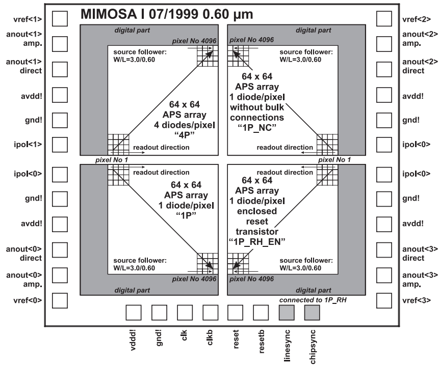
Figure C-3: Simplified structure and pin-out of the MIMOSA I chip (AMS 0.6 μm).
