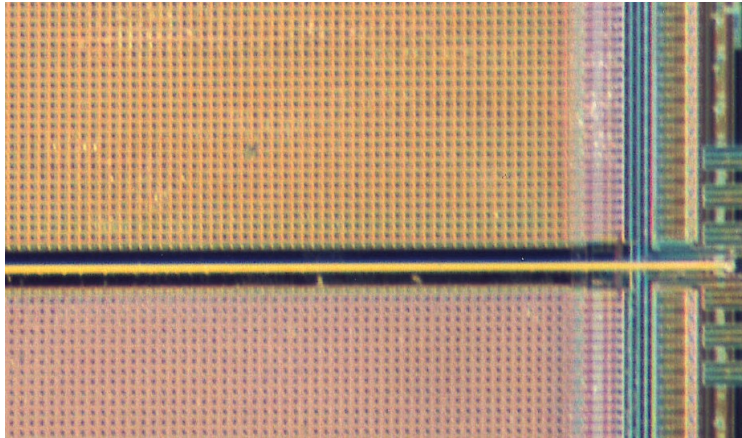
Figure 1-4: Partial die microphotograph of the Monolithic Active Pixel Sensor detector proposed for a highly efficient vertex detector for future collider experiments (MIMOSA I).
