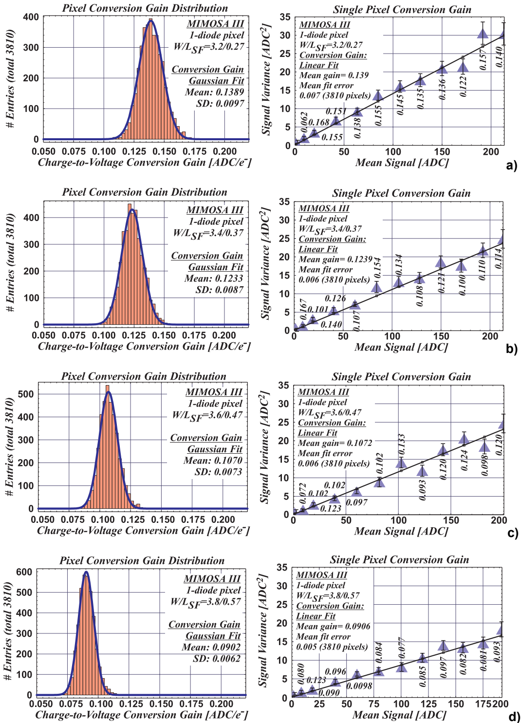
Figure 6-29: Results of charge-to-voltage gain calibration for the MIMOSA III chip obtained by means of the statistical method for different dimensions W/L of the source follower transistor: (a) 3.2/0.27, (b) 3.4/0.37, (c) 3.6/0.47, (d) 3.8/0.57.
