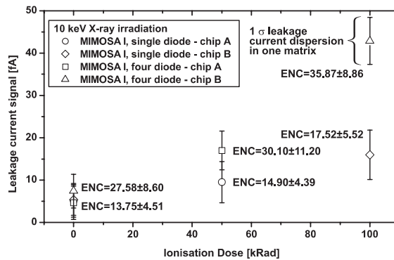
Figure 6-36: Variation of the leakage current and electronic noise measured at 0°C for the single and four diode pixel configurations in the MIMOSA I prototype.
