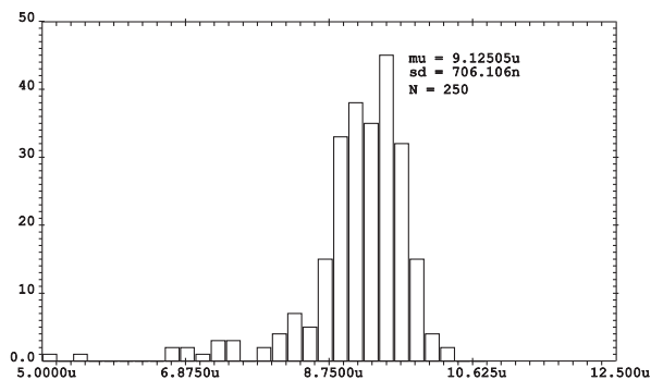
Figure 7-13: Dispersion of the pixel current gain as a result of mismatch variation obtained in the Monte Carlo simulation.
