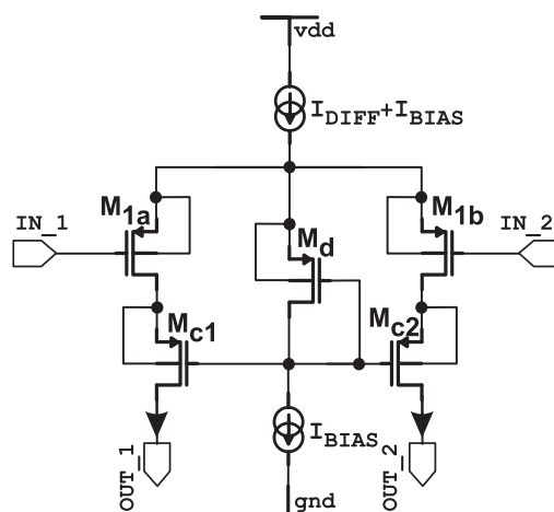
Figure 5-5: Differential cascode with common mode biasing principle.
