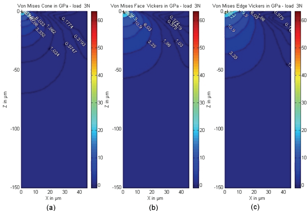
Graph 33: F.E. comparison of Von-Mises distribution between (a) the conical case (equivalent cone), (b) the Vickers' face case and (c) the Vickers' edge case.
