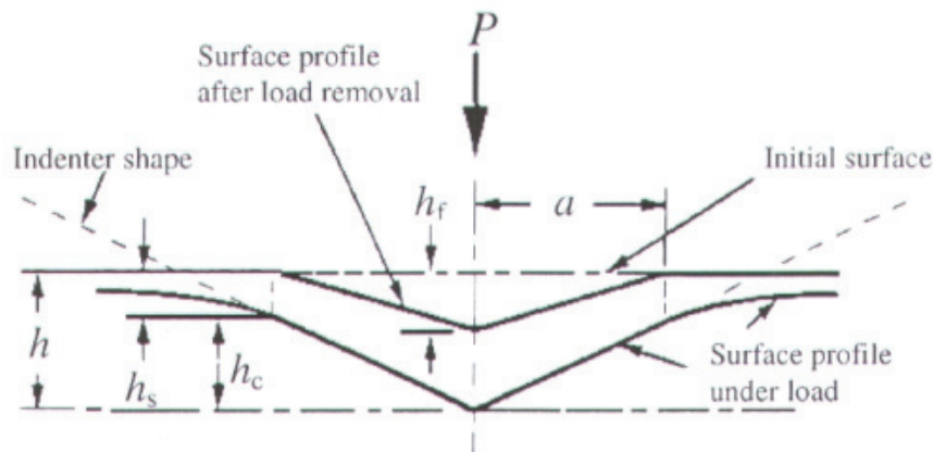
Fig. 54 [92]: Schematic representation of a section through an indentation using a conical indenter.
