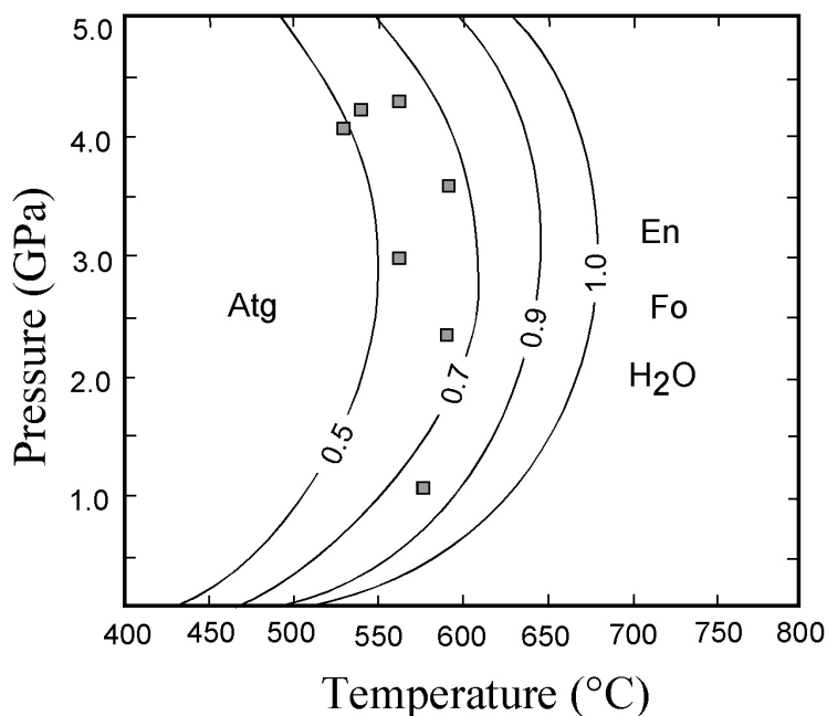
Figure 5.6 - Calculation of the equilibrium antigorite = forsterite + enstatite + \text{H}_2\text{O} in the MSH system for different a_{\text{H}_2\text{O}} conditions ( a_{\text{H}_2\text{O}}=0.5, 0.7, 0.9, 1.0 ), using TWQ (Berman, 1991).
