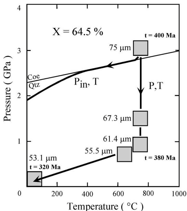
Figure 4.10 - Numerical modelling of the evolution of the size of a coesite inclusion in a pyrope garnet host from the Monts du Lyonnais UHP unit.
