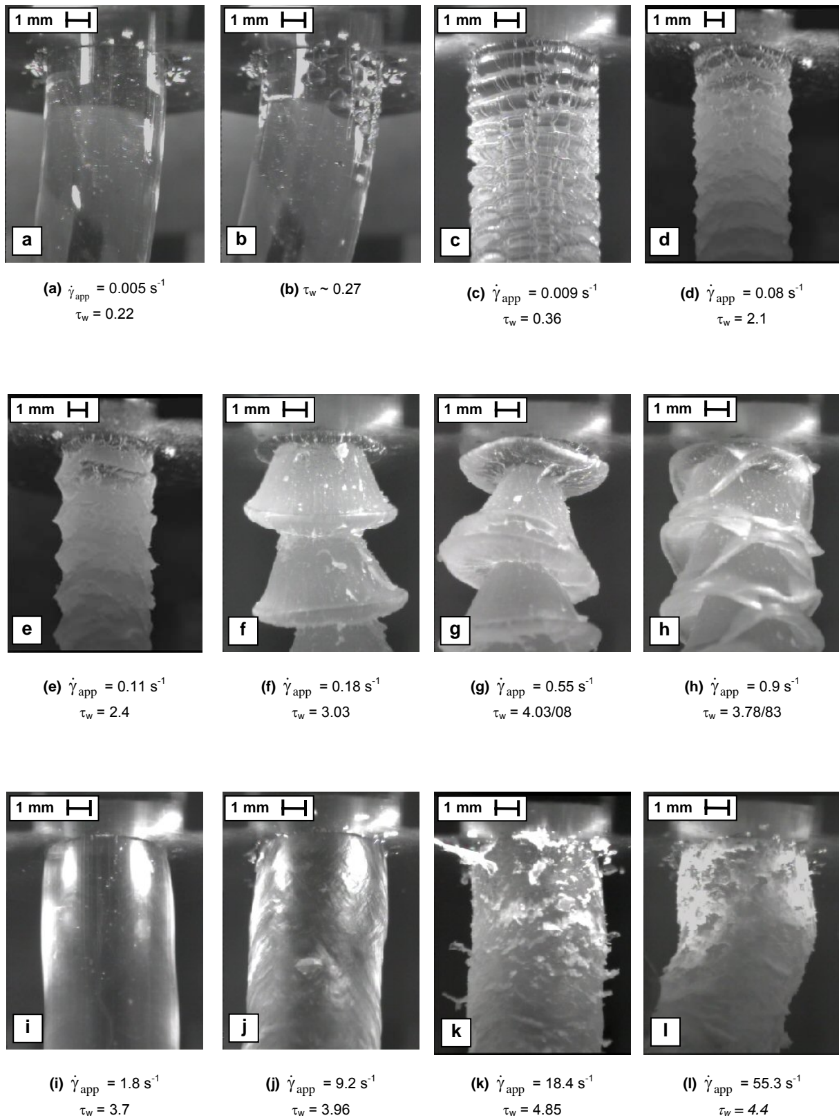
Figure 10: Extrusion at 90°C of SEBS 13%PS at die exit (L/D = 50/5). Apparent shear stress is expressed in 10^5 Pa.
