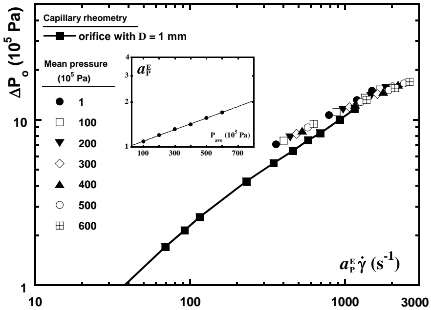
Figure 14: Entrance master flow curve for HDPE at 185 °C using atmospheric pressure as the reference state.
