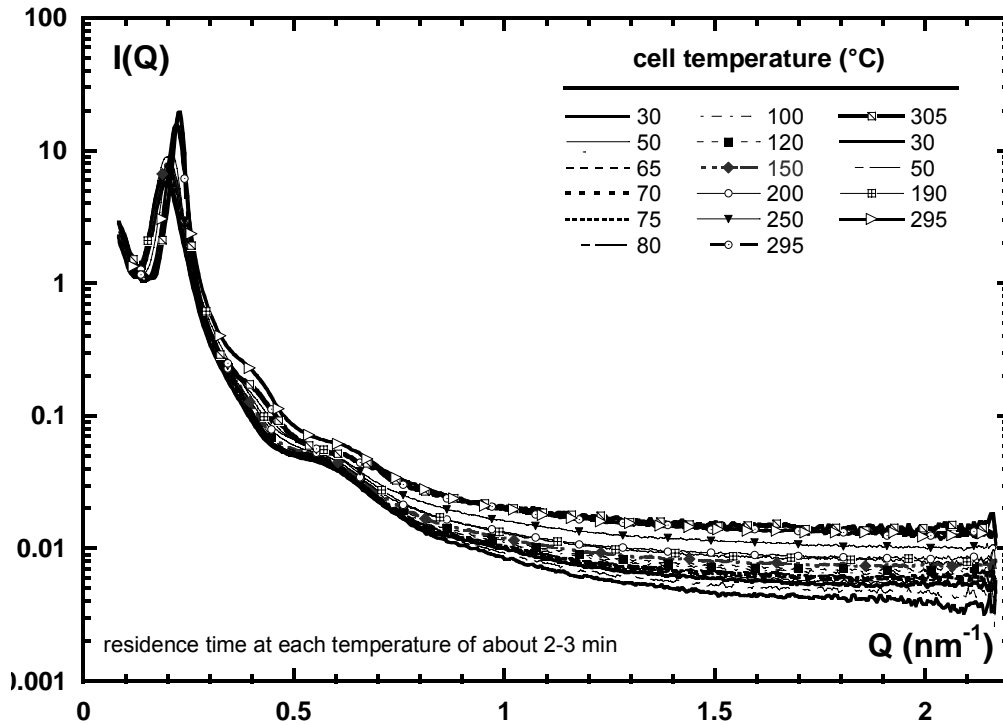
C. 7: Scattered intensity curves for SEBS 30%PS samples obtained by compression molding. Each curve represents a different test temperature.
