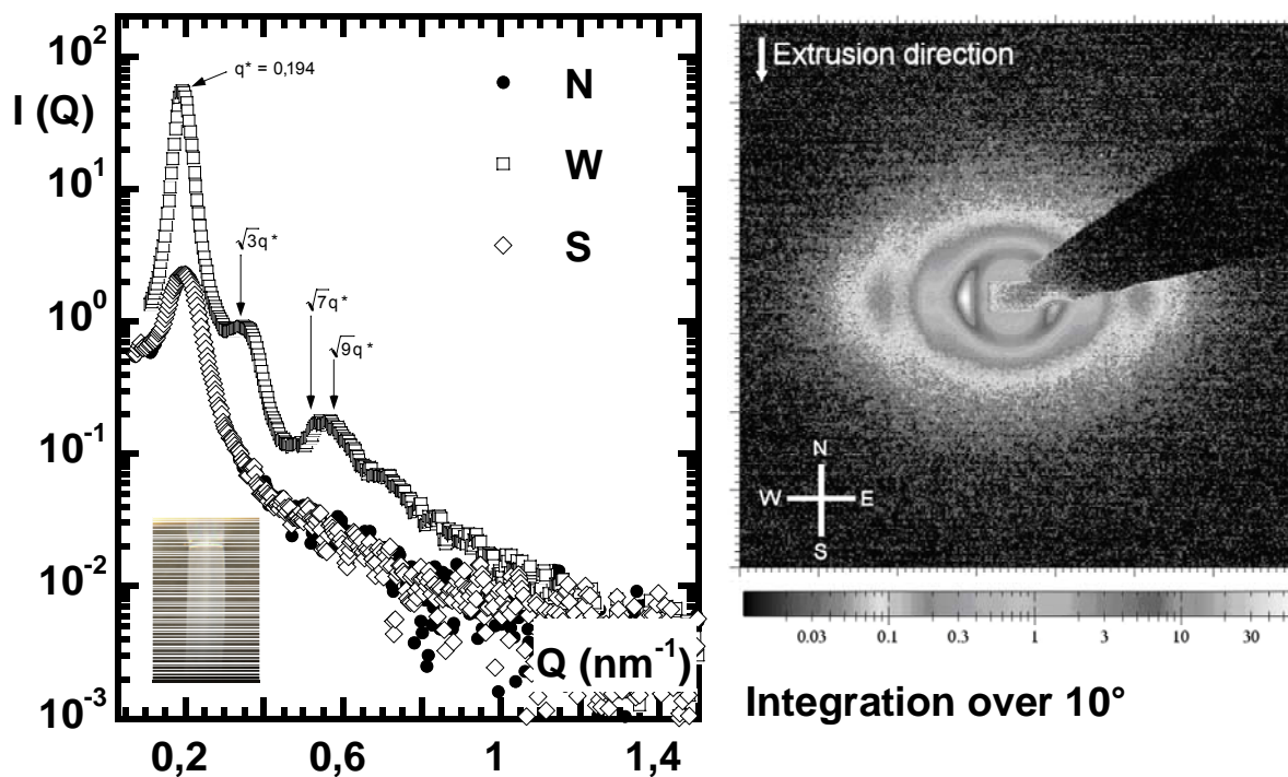
C. 8: SEBS 30%PS extruded at 190°C – 0,005 s -1 – film (not shown). The arrows indicate the theoretical higher order peaks for hexagonally-packed cylinders.
