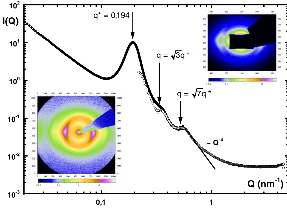
Figure 20: SEBS-1 extruded at 190^{\circ}\text{C} - 0,005 \text{ s}^{-1} – film (not shown). The arrows indicate the theoretical higher order peaks for hexagonally-packed cylinders. Incident beam perpendicular to the extrusion direction. (●) data obtained with a sample-to-detector distance (SDD) of 10 m. (○) SDD of 1.2 m
