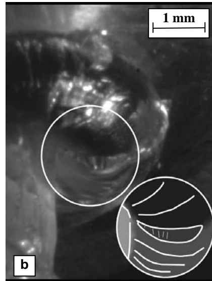
(b) L/D = 50/5 and \Delta P = 80 \times 10^5 Pa. t = 0 sec
