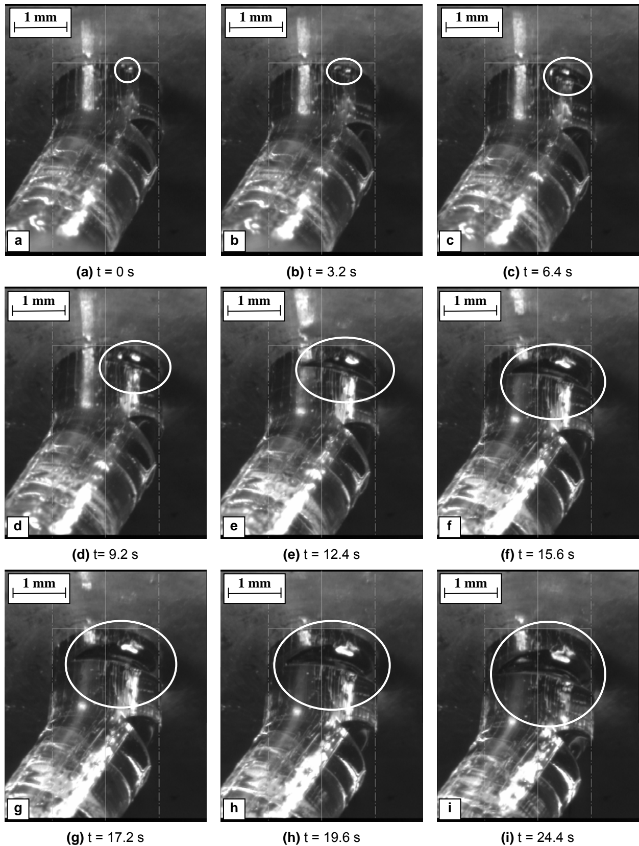
Figure 11: SEBS-2 same extrusion conditions as caption (c) in Figure 9. The experimental conditions were U_p = 0.001 mm s -1 , \Delta P = 6.1 \times 10^5 Pa and a_T \dot{\gamma}_{app} = 0.012 s -1
