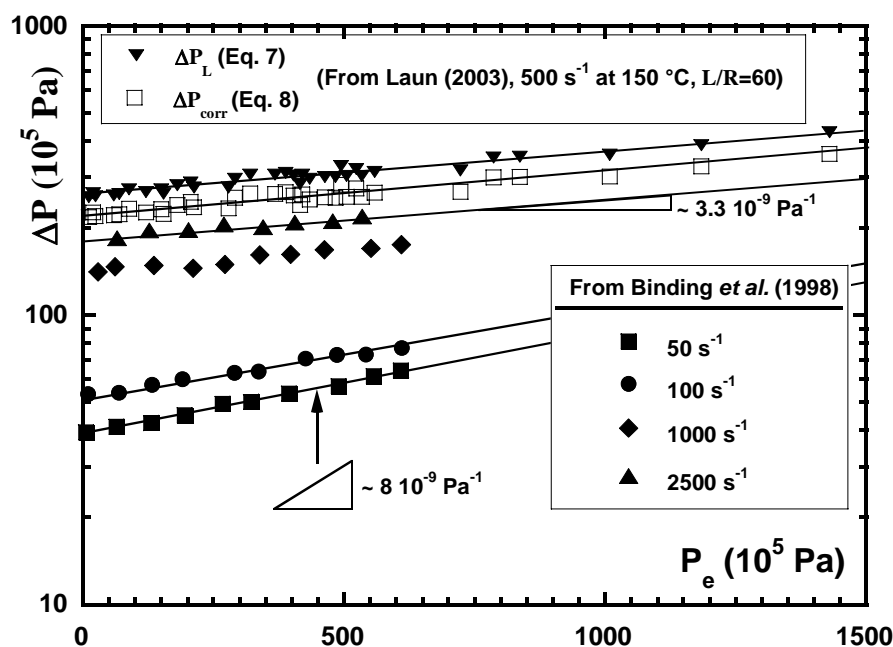
Figure 17: Pressure drop as a function of exit pressure ( P_e ) in long capillaries with L/R of 60 and 50. Data extracted from Binding et al. (1998) and Laun (2003).
