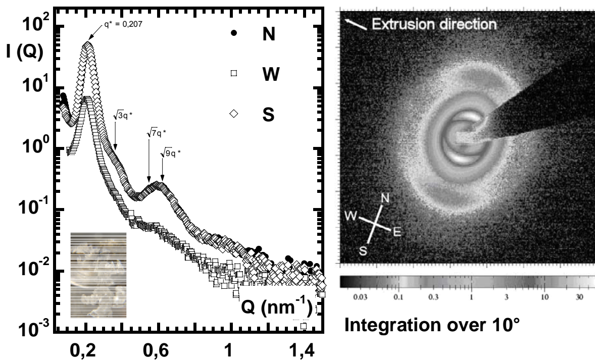
C. 9: SEBS 30%PS extruded at 190°C - 3s -1 through orifice die of 2mm diameter. The arrows indicate the theoretical higher order peaks for hexagonally-packed cylinders.
