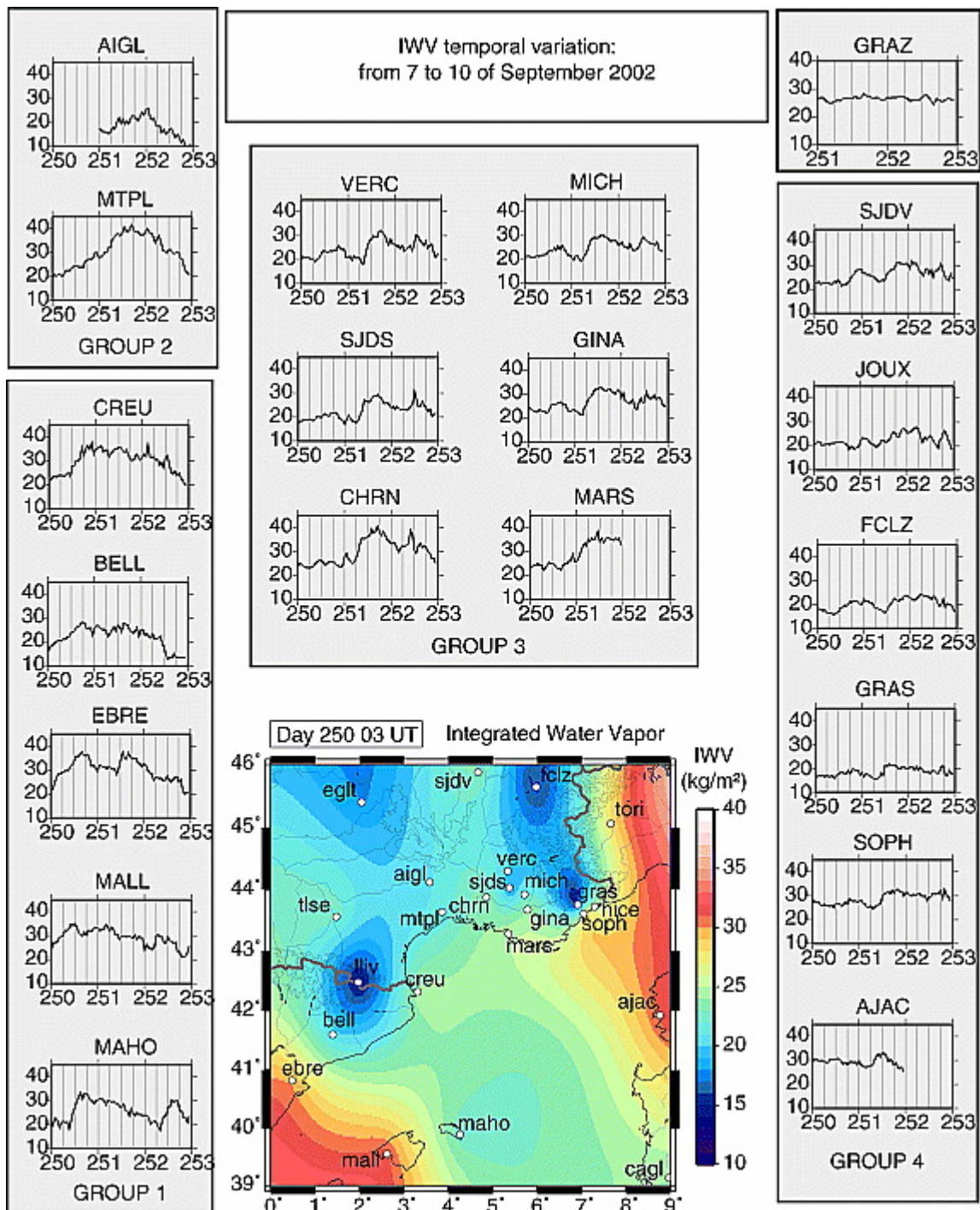
Figure 6. IWV temporal variations (in \text{kg}/\text{m}^2 ) during the 7–10 September for selected GPS stations. The absolute IWV map shown corresponds to the first stage of the event (0300 UTC the 7 September).
