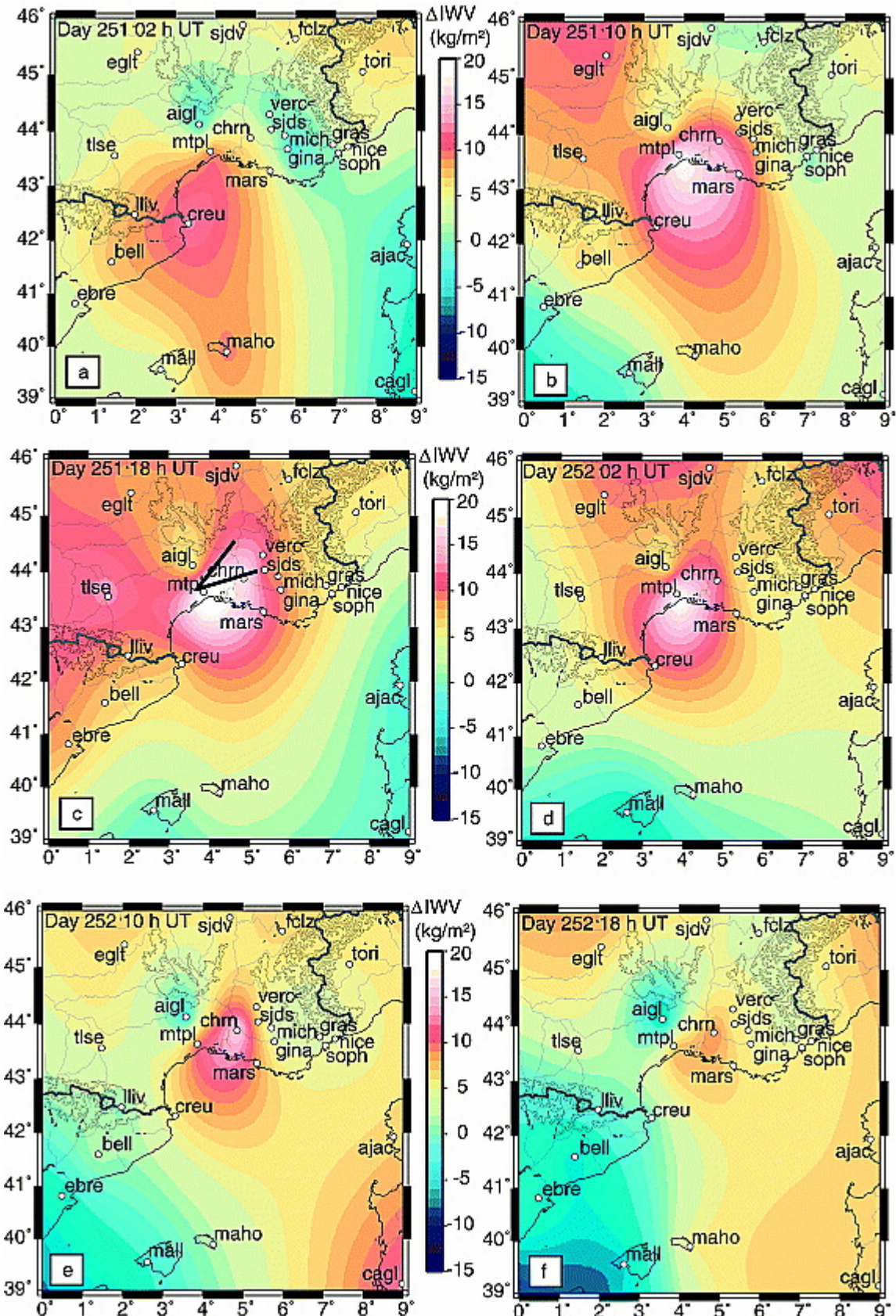
Figure 7. (a–f) IWW maps of the southeast of France relative to day 250 at 1800 UT for each 8 hours from 8 September 0200 UT. The topography is plotted every 1000 m with black lines.
