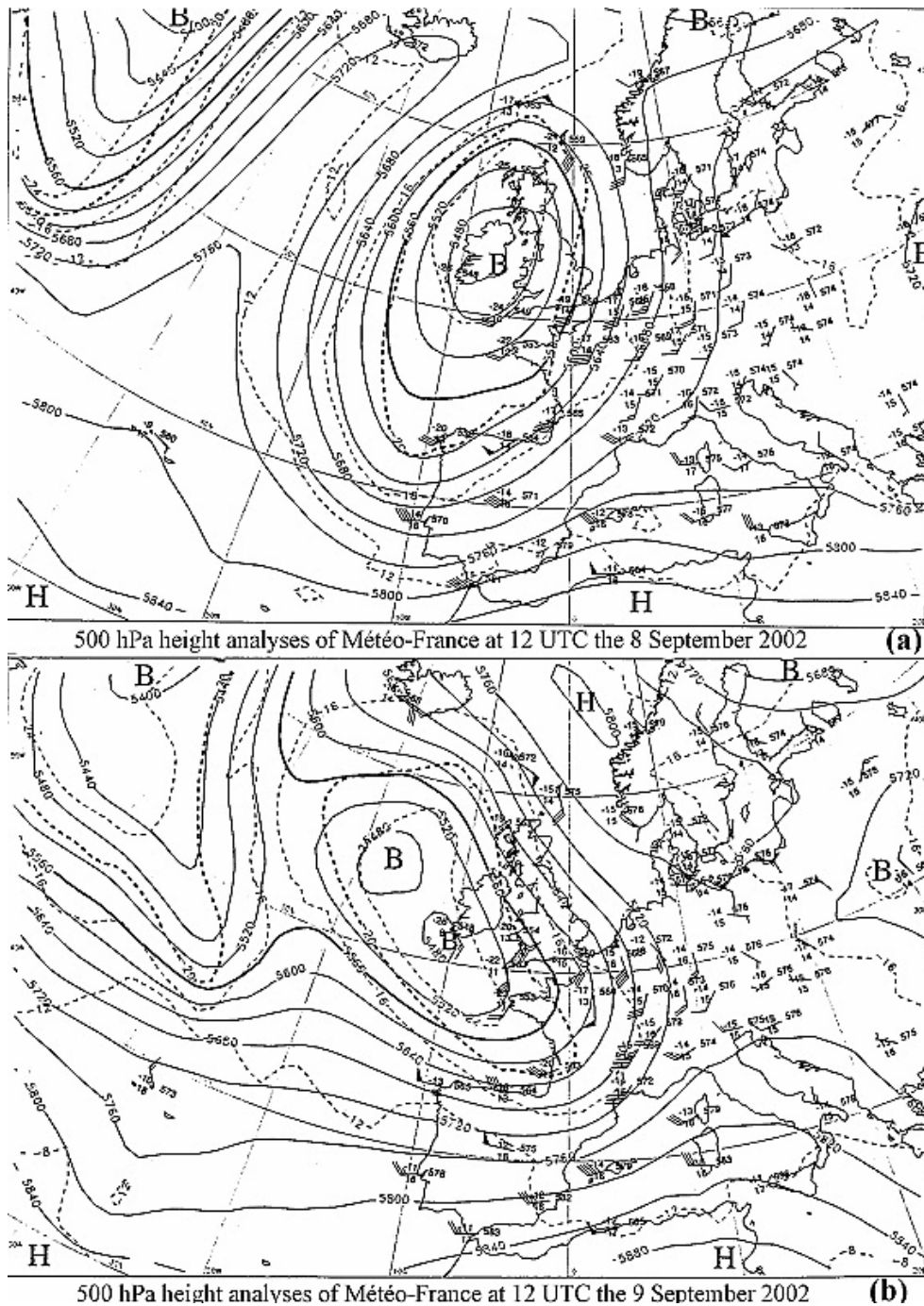
Figure 3. The 500 hPa height analyses of Météo-France (French National Weather Service) at 1200 UTC on (a) 8 September and (b) 9 September. Geopotentials height (in m g p) and temperature (in °C) are represented respectively by solid and dash lines (H for high center of geopotential and B for low center).
