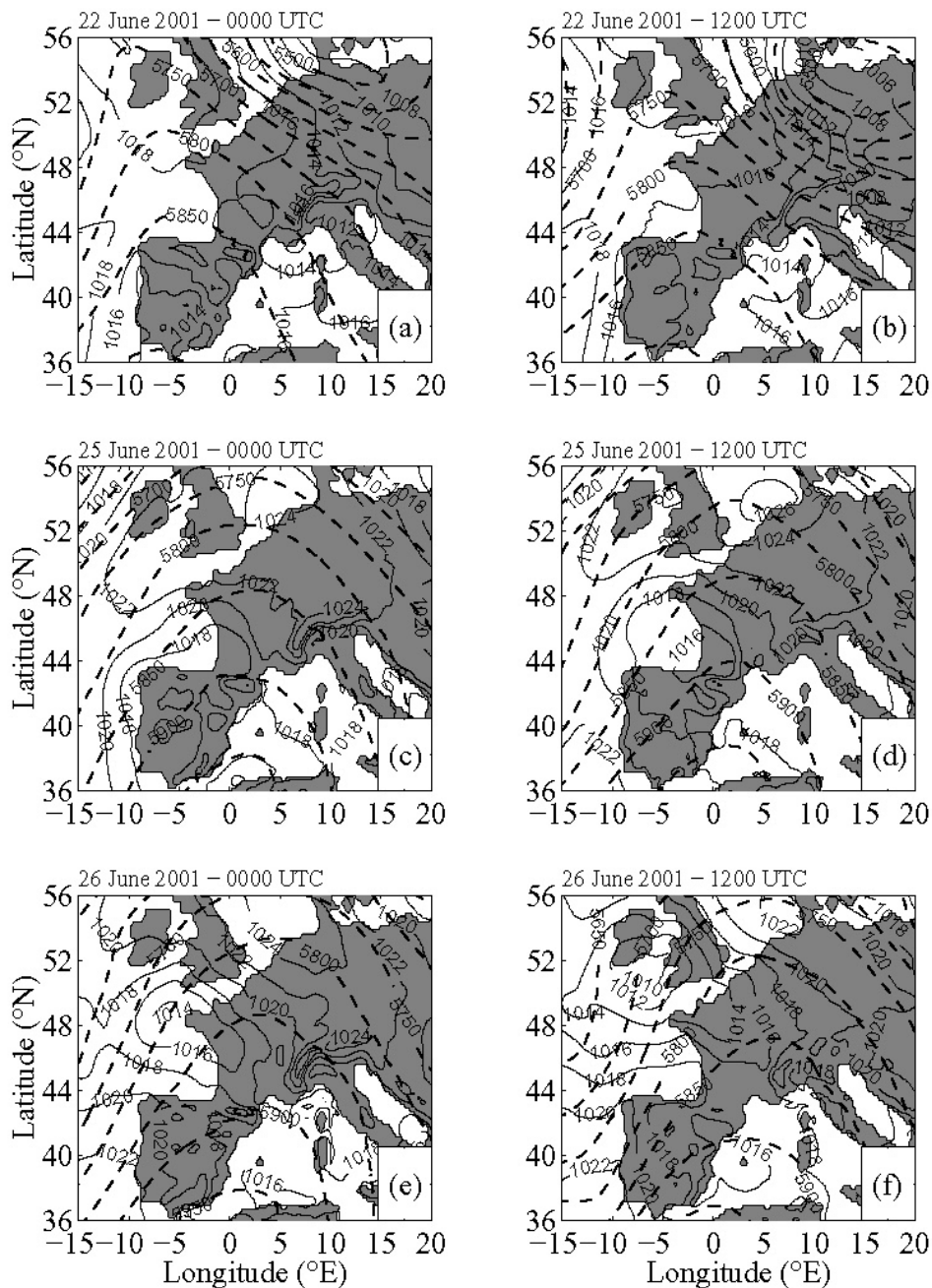
Figure 2 : Synoptic situation in 12-hourly intervals on 22 June 2001 at 0000 UTC (a) and 1200 UTC (b), 25 June 2001 at 0000 UTC (c) and 1200 UTC (d) and 26 June 2001 at 0000 UTC (e) and 1200 UTC (f) from ECMWF analyses. The mean sea-level pressure and 500-hPa geopotential heights are shown with solid (the contour interval is 2 hPa) and thick dashed (the contour is 50 m) lines, respectively.
