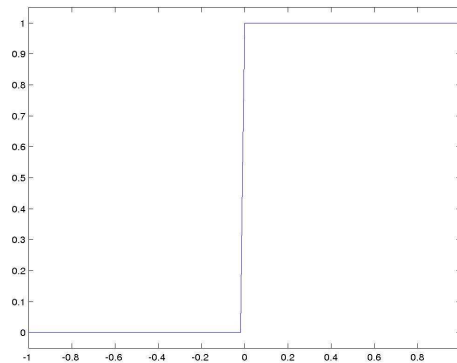
Figure A.19. Graphe de la fonction f_{1,10000,0.01}(x) = \frac{1}{1 + e^{-10000(x+0.01)}} .
