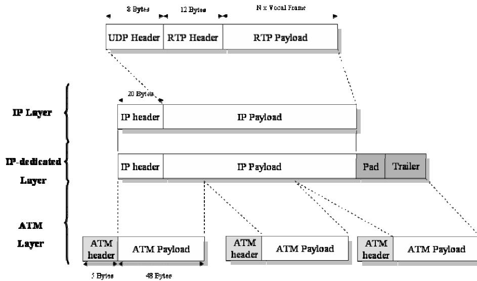
Figure 61 : Encapsulation RTP/UDP/IP/AAL5/ATM
