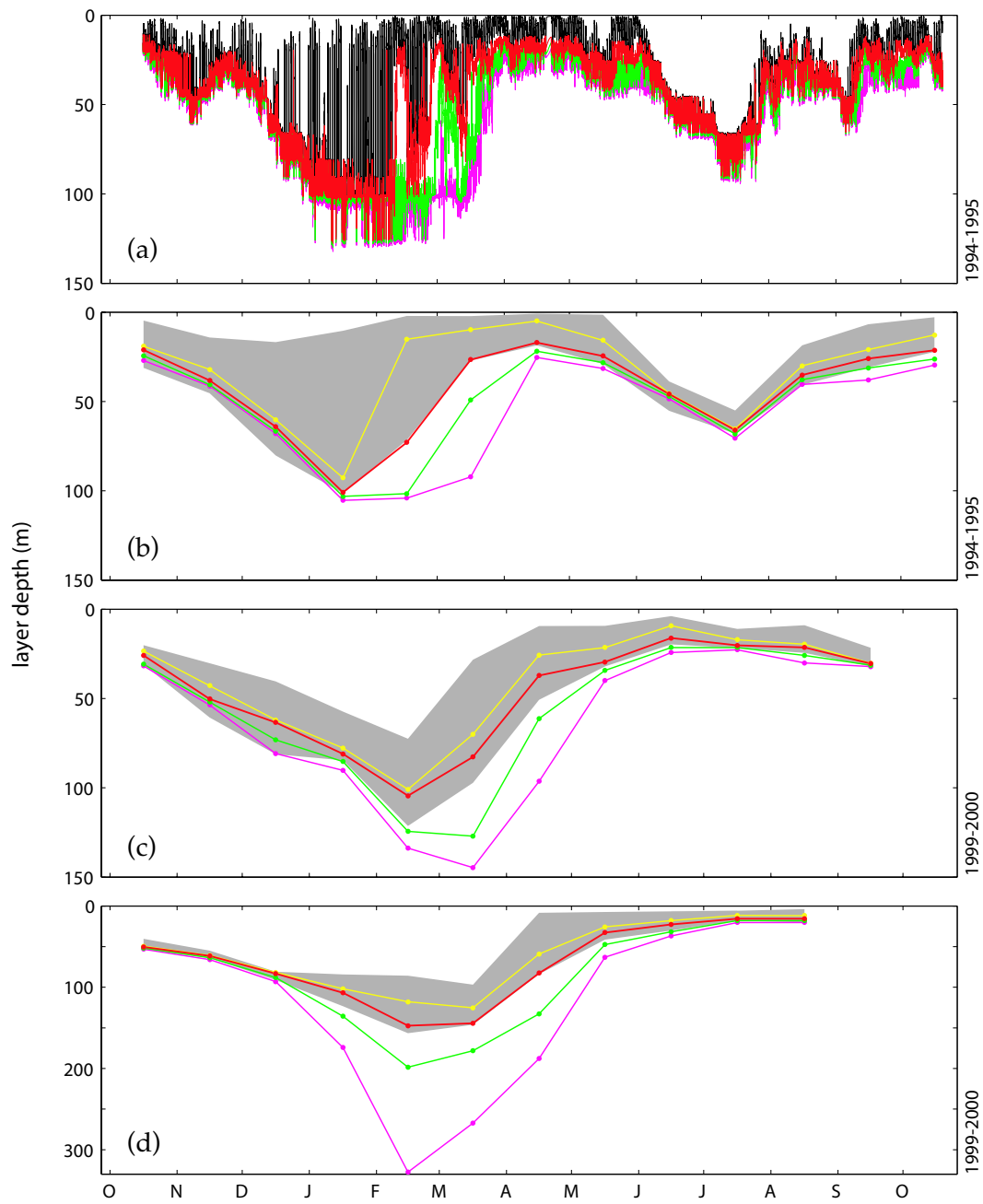
FIG. 22: (a) A time series estimate of the mixing layer depth (black) from a mooring in the central Arabian Sea ( 61.5^{\circ}E , 15.5^{\circ}N ), and the MLD calculated using 3 different threshold temperature criterion from the 10 m temperature : 0.2^{\circ}C (red), 0.5^{\circ}C (green), and 0.8^{\circ}C (pink). (b) The monthly median values of the daily minimum and maximum mixing layer depth (grey shading), the instantaneous mixing layer depth (yellow), and the instantaneous MLD calculated using the same 3 criteria (and same colors) for the mooring in (a). (c) same as (b) for a mooring in the subtropical North Pacific ( 165^{\circ}W , 35^{\circ}N ). (d) same as (b) for the subpolar North Pacific ( 145^{\circ}W , 50^{\circ}N ).
