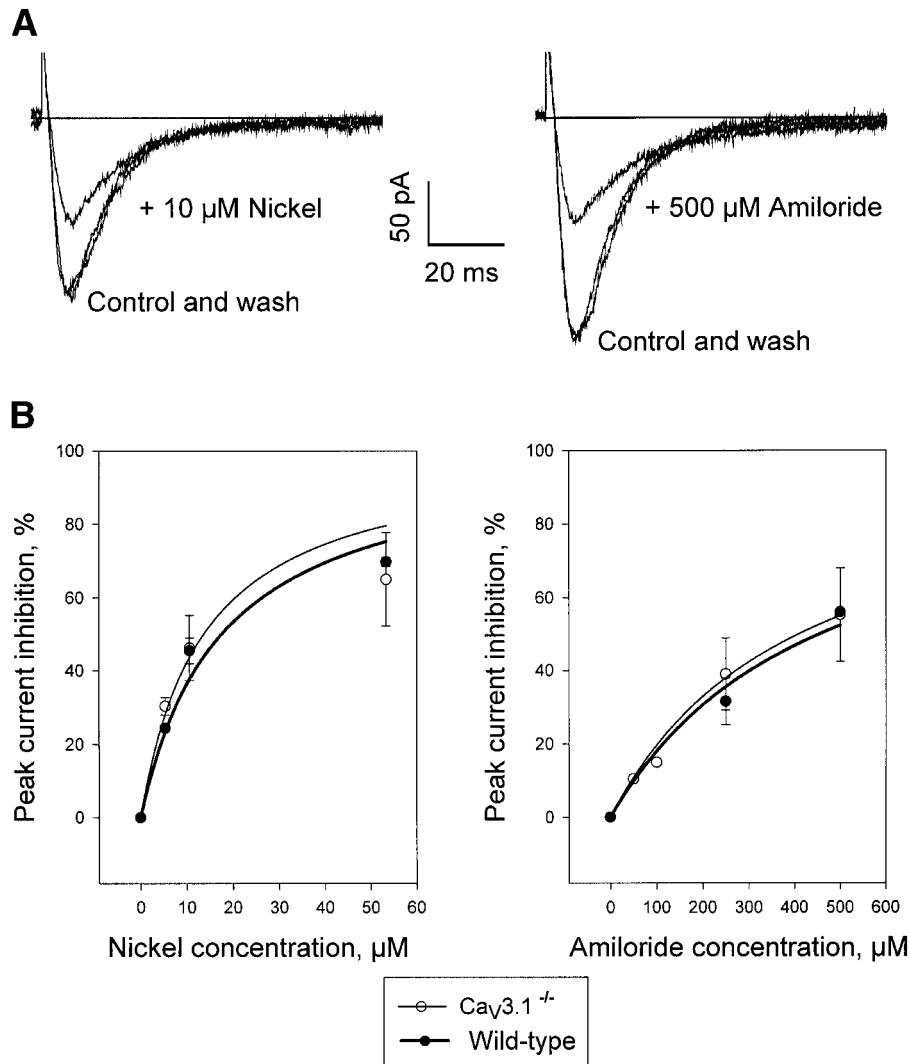
Fig. 5. Amiloride and nickel inhibition of the spermatogenic calcium currents from wild-type and Ca_V3.1 deficient mice. A : Representative current traces showing the current inhibition by nickel and amiloride in spermatogenic cells from Ca_V3.1 deficient mice. HP of -95 mV, test potential of -25 mV. External Calcium concentration is 10 mM. B : Dose-response relationships for the inhibition of peak current
