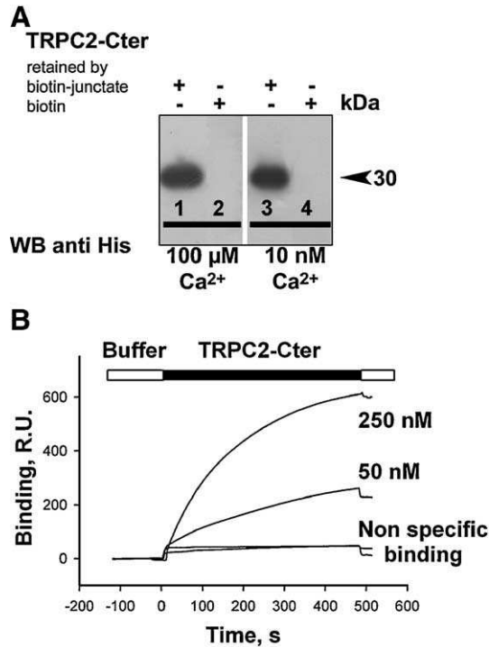
Fig. 4. The junctate amino-terminus interacts with the TRPC2 carboxyl-terminus, and this binding is calcium-independent. (A) Western blot of the bound fractions, showing the binding of TRPC2 on the beads, after pull down of His-TRPC2-Cter with biotinylated junctate-Nter peptide immobilized on streptavidin beads. Biotinylated junctate-Nter peptide was immobilized on streptavidin beads and then incubated with His-TRPC2-Cter. Beads coated with biotin only correspond to a control experiment. His-TRPC2-Cter is immunodecorated with an anti-histidin antibody. This experiment was done in two different calcium concentrations: 100 \mu M (lanes 1 and 2) and 10 nM (lanes 3 and 4). Lanes 1 and 3 show the bound fraction in presence of biotinylated junctate-Nter peptide on beads. Lanes 2 and 4 show the bound fraction on beads coated with biotin only (control). Lanes are extracted from the same gel but rearranged. (B) SPR measurements showing the interaction of TRPC2-Cter (at concentrations of 50 and 250 nM as indicated) with biotinylated junctate-Nter immobilized on the surface of the matrix (total). Control traces (non-specific binding) were obtained with biotin immobilized on the surface of the matrix in a different flow cell and correspond to the non-specific TRPC2-Cter on the surface of the matrix (bulk + NS). The running buffer used contained 50 mM Tris pH 7.4, 150 mM NaCl and 10 nM free calcium concentration.
