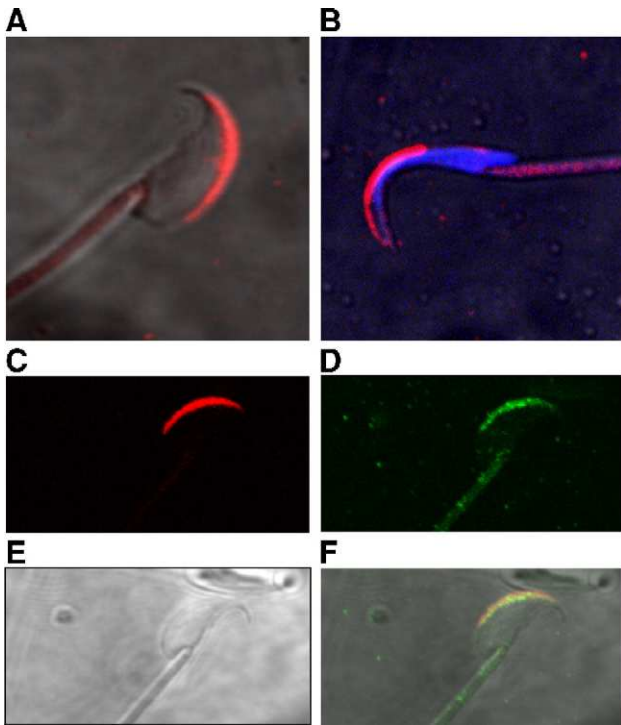
Fig. 2. Junctate is present in the acrosomal crescent of the anterior head. Immunolocalization of junctate in sperm head of mouse (A) and rat (B) evidenced with a junctate-specific antibody. Junctate is localized in the acrosomal crescent of the anterior head. Blue staining in rat sperm head corresponds to the nucleus stained with TOPRO stain. Co-immunolocalization of junctate (C) and IP3R (D) in the same mouse sperm head. (E) Transmitted light image (DIC) and (F) overlay of images presented in panels C–E showing the co-localization of both proteins.
