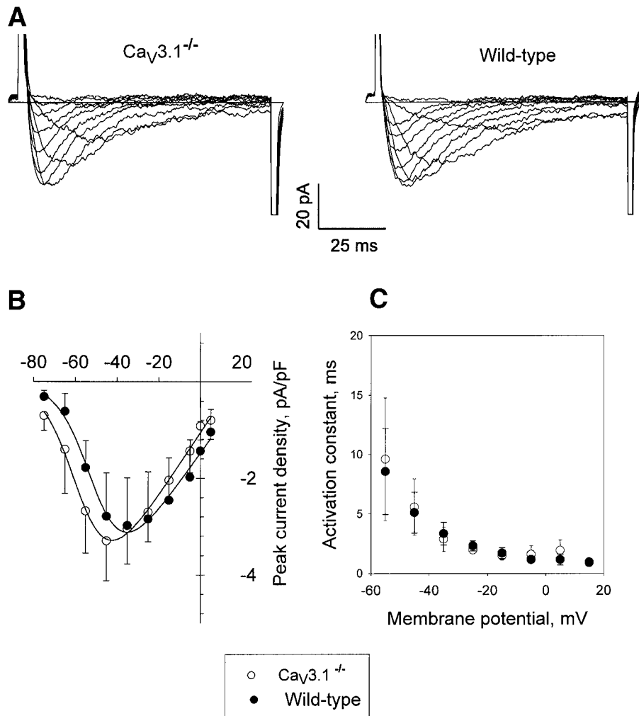
Fig. 3. Activation parameters of spermatogenic calcium current from wild-type and Ca_v3.1 deficient mice. A : Superimposed traces obtained by depolarization from a HP of -105 mV to different test potentials. External calcium concentration, 2 mM. B : Current-voltage relationship (IV curves)—HP -105 mV. (●) Wild-type and
