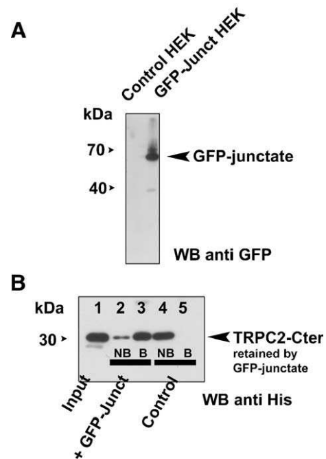
Fig. 3. Junctate and TRPC2-Cter are partners. (A) Expression of GFP-junctate in HEK-293 cells. Western blot using anti-GFP antibody in HEK-293 cells. Lane 1: protein extract from non-transfected cells; lane 2: protein extract from HEK-293 cells transfected with GFP-junctate. Antibody against GFP immunodecorates a protein of around 65 kDa, as expected, since GFP has a molecular weight of 27 kDa and junctate of 40 kDa. (B) Coprecipitation of TRPC2-Cter with GFP-junctate. Protein A beads were coated with an antibody against GFP. Then, two types of cell extracts were incubated with the beads: one from GFP-junctate transfected HEK cells (labeled “GFP-junctate”) and one from non-transfected HEK cells (labeled “control”). Finally, TRPC2 fusion protein (lane 1: Input) was incubated overnight with the beads. Only in the presence of junctate-GFP TRPC2 was immobilized on the beads (lane 3 bound fraction (B)), the supernatant being depleted in TRPC2 fusion protein (lane 2, non-bound fraction (NB)). Lanes 4 and 5 correspond to the beads incubated with cell extract without GFP-junctate. TRPC2 is present in the non-bound fraction (lane 4) and not in the bound fraction (lane 5).
