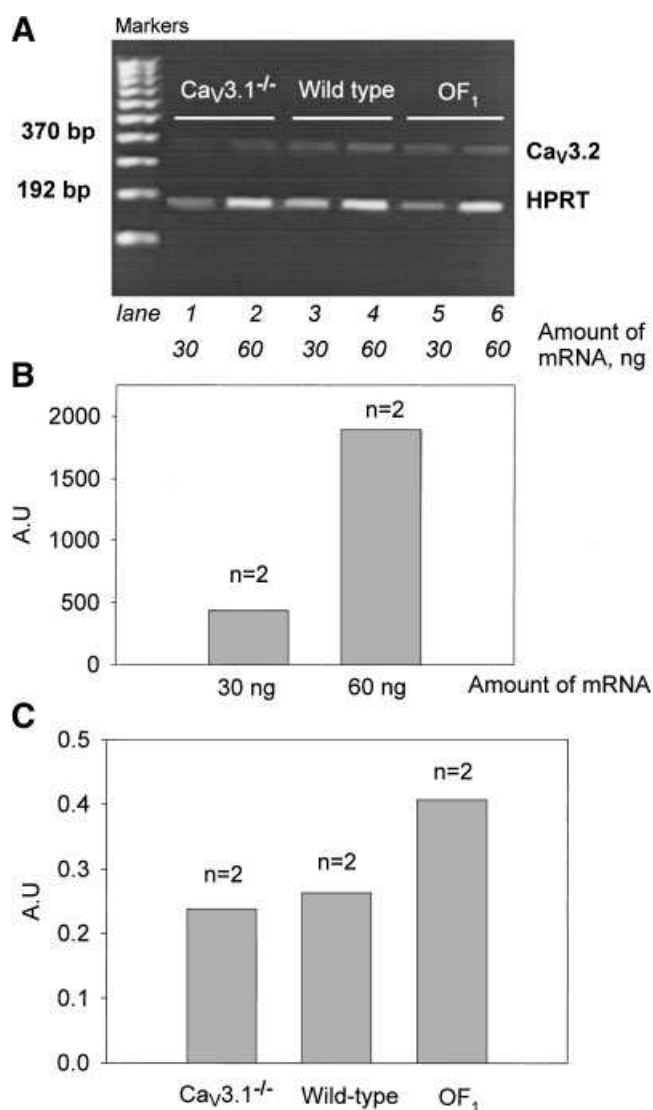
Fig. 6. Semi-quantitative study of Ca_v3.2 expression in spermatogenic cells from wild-type and Ca_v3.1 deficient mice. A: Agarose gel showing the amplification of a 370 bp product by RT-PCR by using specific primers for Ca_v3.2 . During the same experiment, mRNA for HPRT were amplified with specific primers (192 bp). Lanes 1 and 2, mRNA from Ca_v3.1 deficient mice, lanes 3 and 4, mRNA from wild-type mice (cross between 129/SV-Pas and C57BL/6), and lanes 5 and 6, mRNA from OF_1 mice. Two concentrations of mRNA have been amplified to check that we are in the exponential phase of product amplification: 30 ng (lanes 1, 3, and 5) and 60 ng (lanes 2, 4, and 6). The 370 bp product has been sequenced and corresponds to the sequence of Ca_v3.2 mRNA. B: Histogram showing the densities of Ca_v3.2 band measured with a fluorimager™ SI with two concentrations of mRNA (30 and 60 ng) obtained from Ca_v3.1 deficient mice. Average values of two different mRNA extractions. C: Histogram showing the densities of Ca_v3.2 bands measured with a fluorimager™ SI. Values have been normalized by plotting the ratio of the Ca_v3.2 band intensity (30 ng) to HPRT band intensity (30 ng). Average of two different mRNA extractions for the three types of mice.
