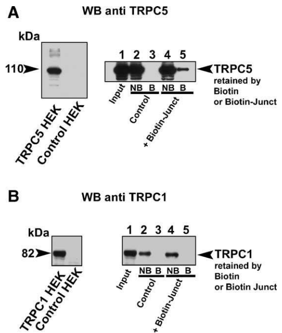
Fig. 5. Junctate binding onto TRPC1 and TRPC5. (A) TRPC5 binds onto the C-terminus of junctate. Left: TRPC5 transiently expressed in HEK-293 cells were specifically evidenced by Western blot. Right: Western blot showing the binding of TRPC5 on the beads, after pull down of TRPC5 with biotinylated junctate-Nter peptide immobilized on streptavidin beads. Biotinylated junctate-Nter peptide was immobilized on streptavidin beads and then incubated with protein extract of cells transiently transfected with TRPC5 cDNA. Only in the presence of biotinylated junctate-Nter TRPC5 was immobilized on the beads (Lane 5 bound fraction (B)); lane 4, non-bound fraction (NB). Lanes 2 and 3 correspond to a same cell extract incubated with beads coated with biotin only (control experiment). In the control experiment, TRPC5 is not retained (lane 3 bound fraction (B)); lane 2, non-bound fraction (NB). Lane 1 corresponds to cell extract (input). TRPC5 is immunodecorated with an anti-TRPC5 antibody. (B) TRPC1 does not bind onto the C-terminus of junctate. Left: Western blot showing expression of TRPC1 in HEK cells transiently transfected with TRPC1 cDNA. Right: Western blot showing the absence of binding of TRPC1 on the beads, after pull down of TRPC1 with biotinylated junctate-Nter peptide immobilized on streptavidin beads. The protocol is identical as presented in panel A for TRPC5.
