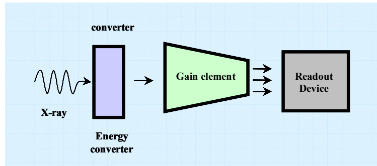
Figure 4-9: Schematic principle of an X-ray detector
