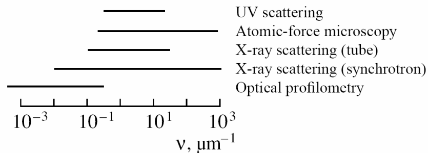
Figure 2-2: Typical spatial frequency ranges accessed by presently existing methods of investigation of surface roughness.
