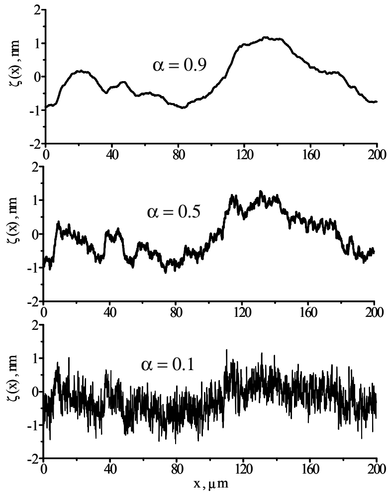
Figure 3-11: Rough surfaces of the same rms height \sigma = 0.5 \text{ nm} and the same correlation length a = 20 \text{ }\mu\text{m} but of different roughness exponent \alpha , see ref. [65].
