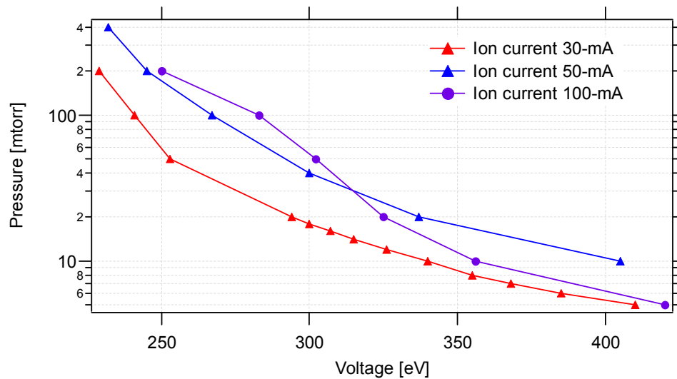
Figure 4-5 Paschen curves obtained for different target current.
