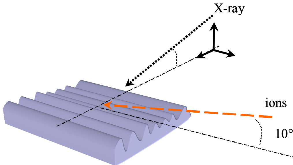
Figure 6-14: X-ray Scattering geometry with ripples formed in accordance to the BH model.
