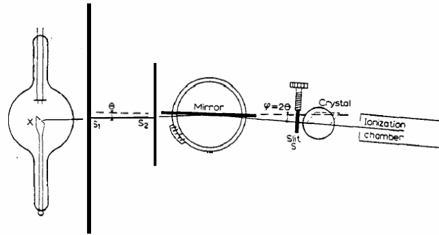
Figure 1-3: The apparatus used by Compton for studying the total reflection of X-rays (taken from his Nobel lecture 3 ).
