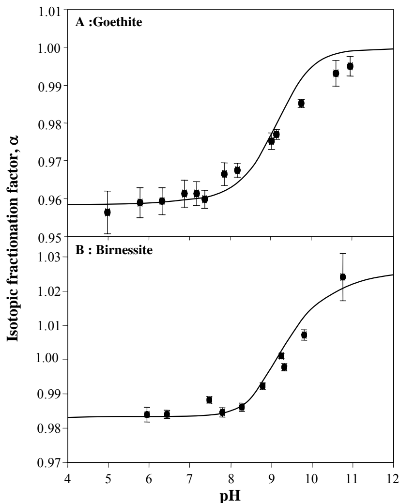
Figure 7: Modeling (solid line) of boron isotopic fractionation at the surface of goethite (A) and birnessite (B) taking an \alpha_{IV-III} value equal to 0.965 at 25°C.
