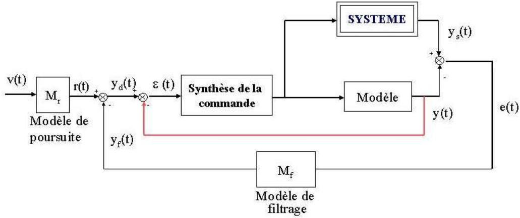
Figure 4.1 : La structure IMBC
