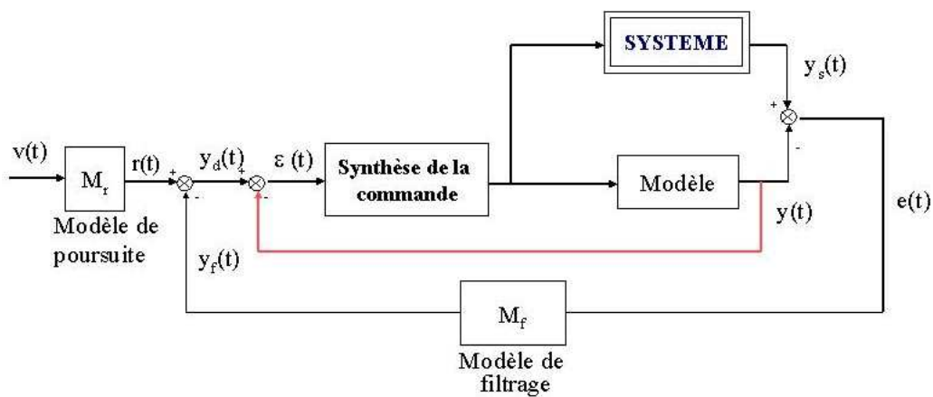
Figure 2.3 : La structure IMBC
