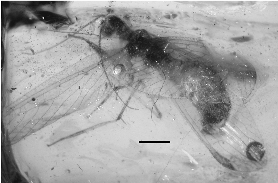
Fig. 19. Eorhachiberotha celinea sp. n., holotype PA 346 (1), photograph of left lateral view (scale bar represents 1 mm).
