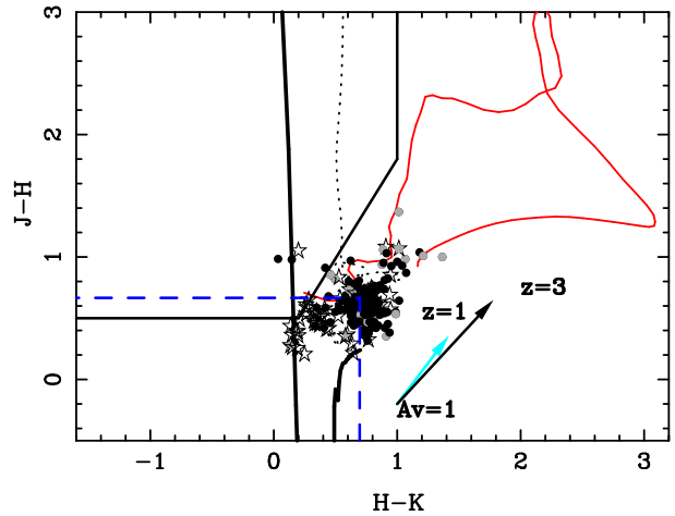
Fig. 8. Location of objects brighter than H = 22.5 in the J-H vs H-K color-color diagram for Abell 1835 (black dots). Special symbols are used for SExtractor stars ( flag_* > 0.95 , open stars) and EROs (grey dots). Predicted colors for an elliptical cluster galaxy are shown with dashed lines, and the direction of reddening is indicated by an arrow. Evolutionary tracks are overplotted as in Fig. 1, to facilitate the comparison: E galaxy (grey solid line), a low-metallicity starburst (thick solid black line) and a local starburst from Kinney et al. 1996 (dotted line). Error bars are typically \leq 0.1 mags for these objects.
