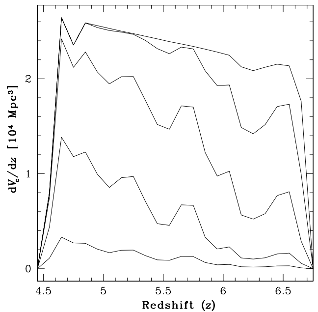
FIG. 9.—Redshift distribution of our survey volume. The curves, from top to bottom, represent the redshift distribution of subsurveys down to limiting luminosity \log_{10} L = (43.5, 43, 42.5, 42, 41.5) ; for yet lower values of the limiting luminosity, the curves have the shape of the bottom curve, but are scaled down (see Fig. 10).
