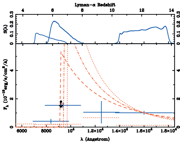
FIG. 3.— Top : Relative efficiencies of the filter+instrument used in our photometric observations. From left to right : WPC2-F814W, ACS-F850LP, and NICMOS-F160W. Bottom : Spectral energy distribution of image a uncorrected for lensing magnification. Photometric points are indicated by blue crosses, and the 3\sigma point source detection limits are indicated by horizontal dashed red lines below each data point. The nondetection of the continuum in the LRIS 9000–9300 Å window is indicated by the black arrow. Red dashed lines correspond to power-law SEDs [with f \propto \lambda^{-\alpha} for \lambda/(1+z) > 1216 Å and f = 0 otherwise] with slope indices (from bottom to top at 1.2 \times 10^4 Å) of \alpha = 3, 4, and 5 . The available data are consistent with a neutral hydrogen break in the interval 9250–9850 Å corresponding to 6.6 < z < 7.1 .
