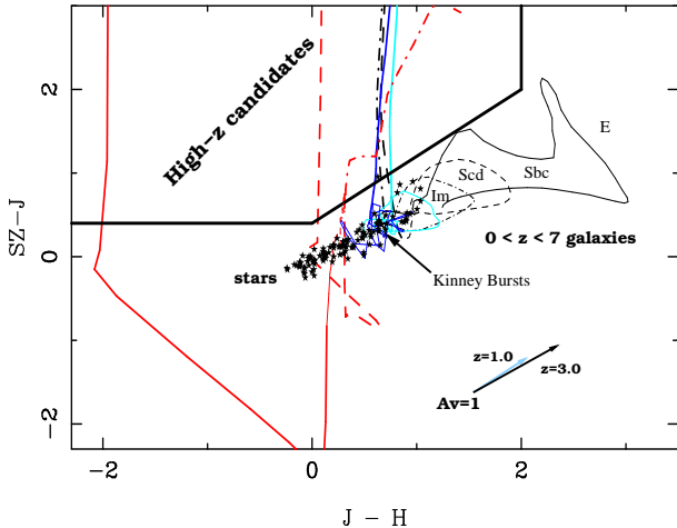
Fig. 2. SZ - J versus J - H s color-color diagram (Vega system) showing the position expected for different objects over the interval of z \sim 0 to 8.5. Thin and thick lines display models below and above z = 7 respectively. Models displayed and general comments are the same as in Fig. 1. The position of stars and normal galaxies up to z \leq 7 are shown.
