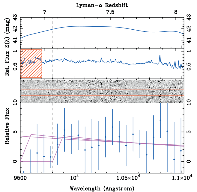
FIG. 5.—NIRSPEC spectrum for image a in the wavelength region 9500 Å–1.1 \mu m. Top : Relative sensitivity of NIRSPEC in the configuration used derived from three independent flux calibration stars. Adequate sensitivity is available over the entire range. Middle : Observed spectrum of one of these standards, Feige 110 illustrating a priori the absence of any strong atmospheric features in the reduction. The red hatched rectangle indicates the region where variable atmospheric absorption is expected (Massey & Gronwall 1990). Bottom : Flux-calibrated binned spectrum for image a . Error bars include the effect of wavelength-dependent OH emission. Curves represent UV SEDs consistent with the photometry (Fig. 3) spanning the range 6.6 < z < 7.1 . The absence of significant flux below 9800 Å suggests a redshift at the upper end of this range, i.e., z \simeq 7 .
