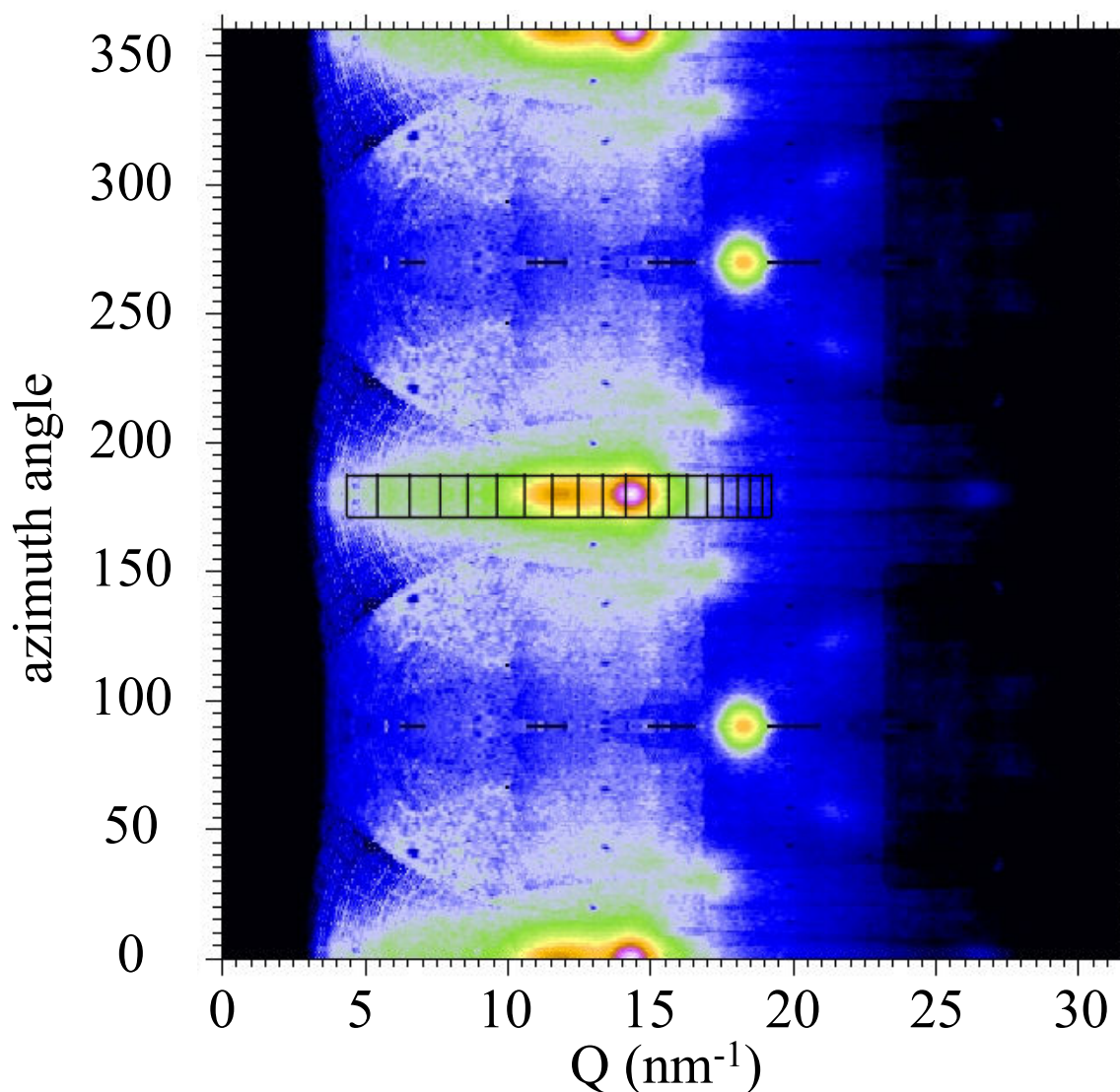
Figure 55 Cake-regrouped neutron fibre diffraction pattern of H 2 O-humidified silk superimposed with the area covered by the IN16 detectors (boxes on the equator). The IN16 multidetector tubes are evenly spaced in 20.
