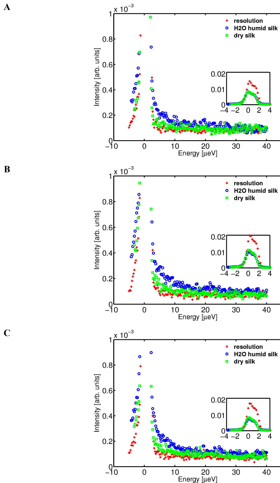
Figure 48 High energy resolution spectra obtained on IN10b for different humidity conditions (H 2 O-humid, dry) for different Q range (centered at Q = 6.8 \text{ nm}^{-1} (A), Q = 13.2 \text{ nm}^{-1} (B) and Q = 18.3 \text{ nm}^{-1} (C)). IN10b instrument. Analysed wavelength \lambda = 0.627 \text{ nm} . T = 290 \text{ K} . Humid silk obtained by storing overnight in H 2 O-humid saturated atmosphere at room temperature. In-situ drying during several minutes pumping at 300 \text{ K} .
