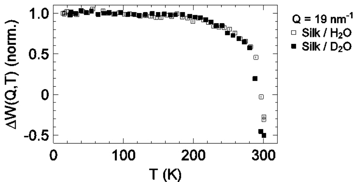
Figure 54 Difference signal of H 2 O and D 2 O humid silk minus native dry silk. The difference spectra are shown only at a single Q of 19 nm -1 . The intensities before subtraction were measured at "fixed energy window" scan centred at zero energy transfer (Figure 51).
