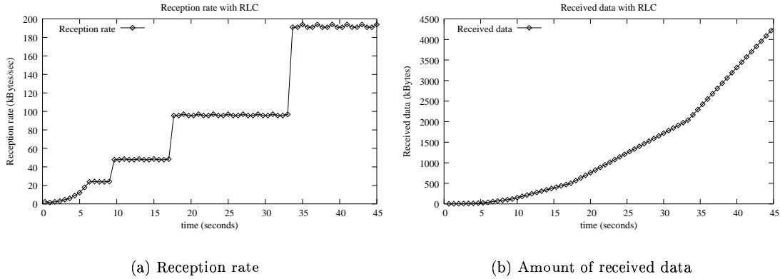
Figure 12.3: RLC measurements.
