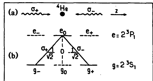
FIG. 1. (a) Two counterpropagating \sigma_+ and \sigma_- polarized laser beams interact with ^4\text{He} atoms on the 2^3S_1 - 2^3P_1 transition. (b) The Zeeman sublevels, and some useful Clebsch-Gordan coefficients. Since the e_0 \leftrightarrow g_0 transition is forbidden, all atoms are pumped into g_+ and g_- after a few fluorescence cycles. These two levels are coupled only to e_0 , and a closed three-level \Lambda configuration is realized (solid lines).
