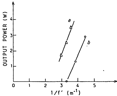
Fig. 6. Vertical axis: output power of the lamp pumped laser for a short cavity and a plane output mirror ( T=1\% ). Horizontal axis: inverse focal distance f' of the crystals (for definition, see text). (a) for LMA:Cr, Nd (crystal A), (b); for LMA:Nd (crystal B).
