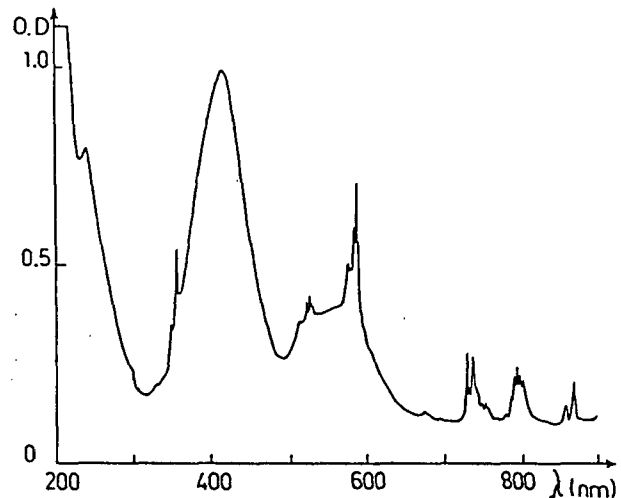
Fig. 1. Absorption spectrum of the \text{LMA}:\text{Nd, Cr} crystal obtained on a Kontron Uvicon 860 double beam spectrometer. The unpolarized beam of the spectrometer was directed along the a -axis of the sample, whose thickness was 2.65 mm.
