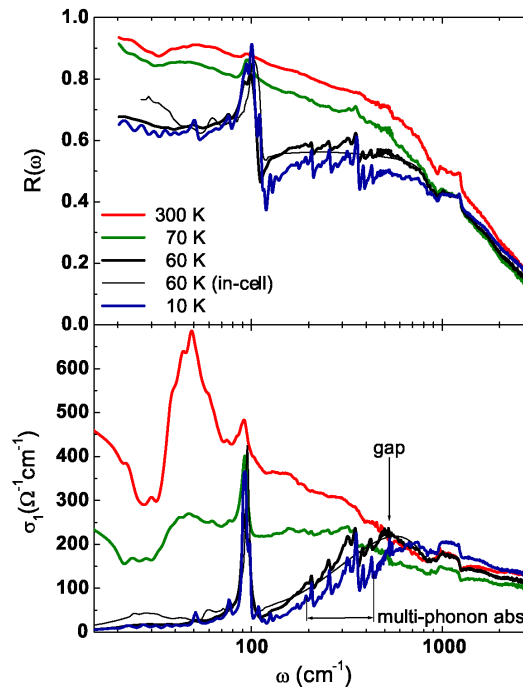
Figure 8.1: The reflectivity (upper panel) and conductivity (lower panel) spectra of \text{BaVS}_3 at ambient pressure for selected temperatures. The position of the gap is indicated by arrow. To test the reliability of the high-pressure data (see below), the 60\text{ K} curve was also measured in the pressure cell at ambient pressure.
