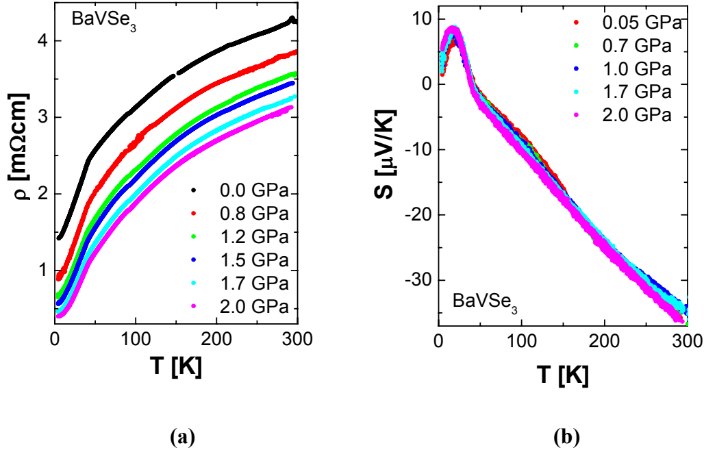
Figure 6.6: (a) Resistivity and (b) thermoelectric power of BaVSe 3 in the temperature range 4 – 300 K, under pressures up to 2 GPa.
