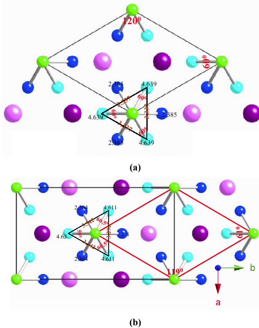
Figure 3.7: Projection view, along the c -direction, of the crystal structure of BaVS_3 (a) in the hexagonal structure at room temperature (b) in the orthorhombic structure at 100 K. Vanadium atoms are green, barium atoms are violet (light at \frac{1}{4}c dark at \frac{3}{4}c ) and sulfurs atoms are blue (light at \frac{1}{4}c dark at \frac{3}{4}c ). The vanadium-sulfur distance is marked by black numbers. The in-plane distances of sulfur are denoted by brown numbers. All the distances are given in Angstroms. The red numbers refer to in-plane angles between sulfur or vanadium atoms.
