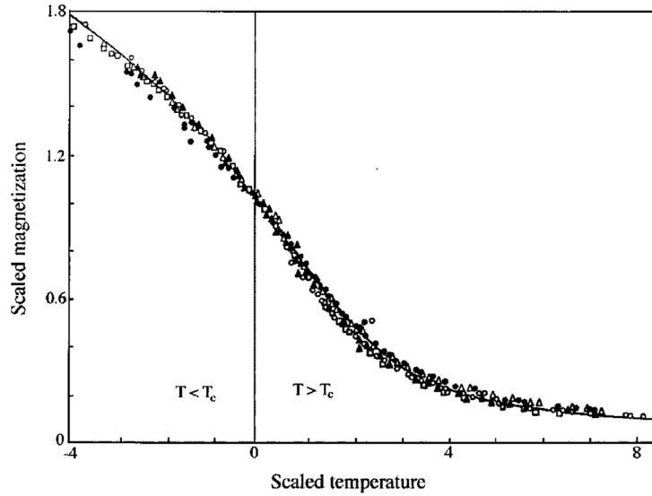
Figure 5.4: An example of a scaling analysis in the case of a classical phase transition. Experimental magnetization M(H, T) data for five completely different materials (CrBr 3 , EuO, Ni, YIG, and Pd 3 Fe) plotted in their scaled forms. Despite their differences, the data for all materials fall onto a single scaling function, which is that calculated for the d = 3 Heisenberg model (Milošević and Stanley, 1976).
