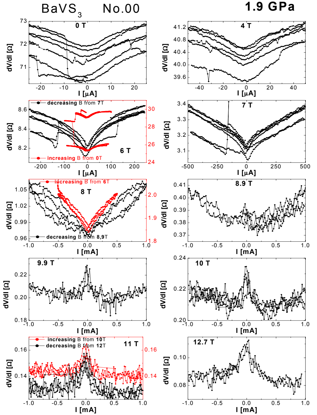
Figure 5.21: The dV/dI characteristics, at T=4 K, as a function of current for several magnetic fields, showing the instability of the system to the current. The black and red colors are related to the direction of the change of the field before recording the characteristic.
