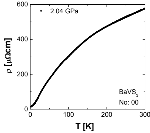
Figure 5.2: The resistivity at the pressure of 2.04\text{ GPa} shows a metallic behavior in the whole measured temperature range. The MI transition is completely suppressed.
