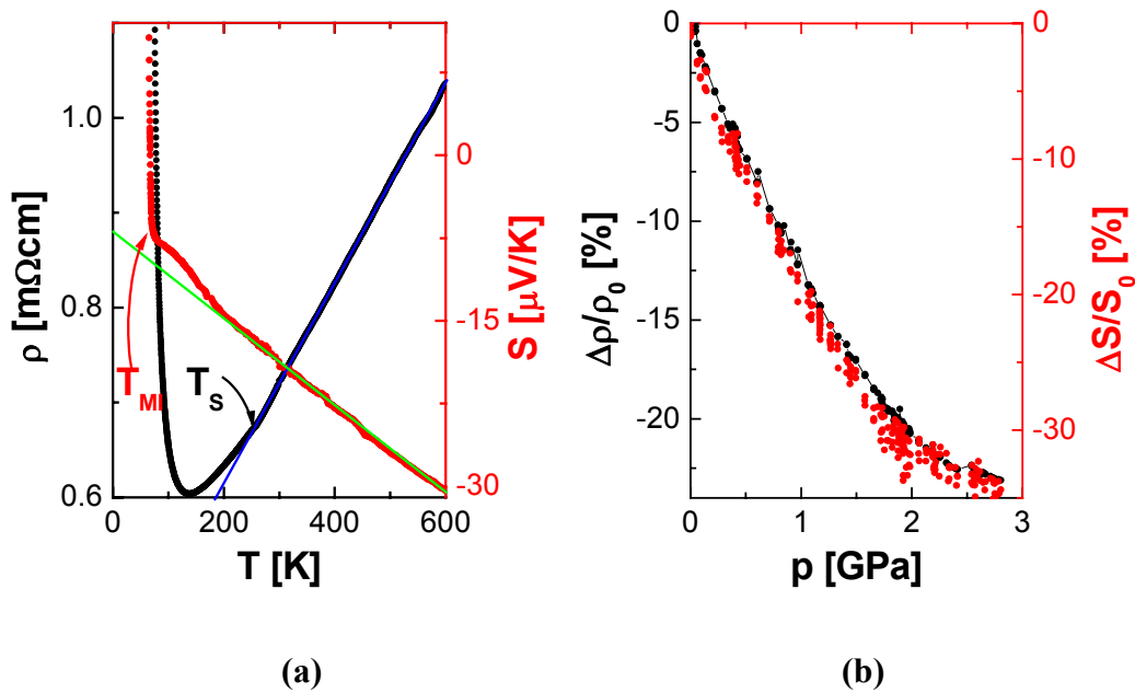
Figure 7.1 (a) Thermoelectric power and electrical resistivity of \text{BaVS}_3 in the 0-600 K range. Above T_S = 240 \text{ K} , both the electrical resistivity and the thermoelectric power show linear temperature dependence indicated by blue and green eye-guide lines. (b) The pressure dependence of the relative change of the resistivity (black circles) and of the thermoelectric power (red circles) at room temperature. Note the difference between the right and left hand scales.
