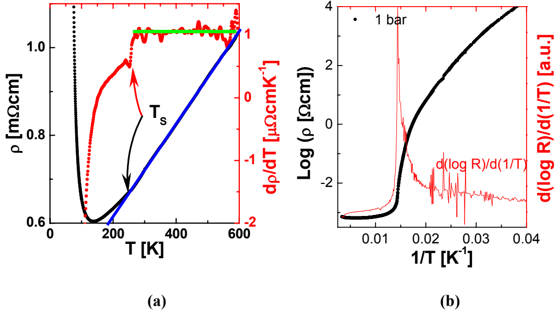
Figure 4.1: Black lines describe the temperature dependence of electrical resistivity of BaVS 3 shown on: (a) the linear scale in the 0-600 K range revealing the linear temperature dependence above T_S , (b) the Arrhenius plot giving insight into the electrical properties of the insulating phase. Red scales are related to (a) temperature derivative and (b) logarithmic derivative of the electrical resistivity disclosing the weak change of slope of resistivity at T_S , and the temperature of the MI transition, respectively. The green and the blue lines are guides to the eye.
