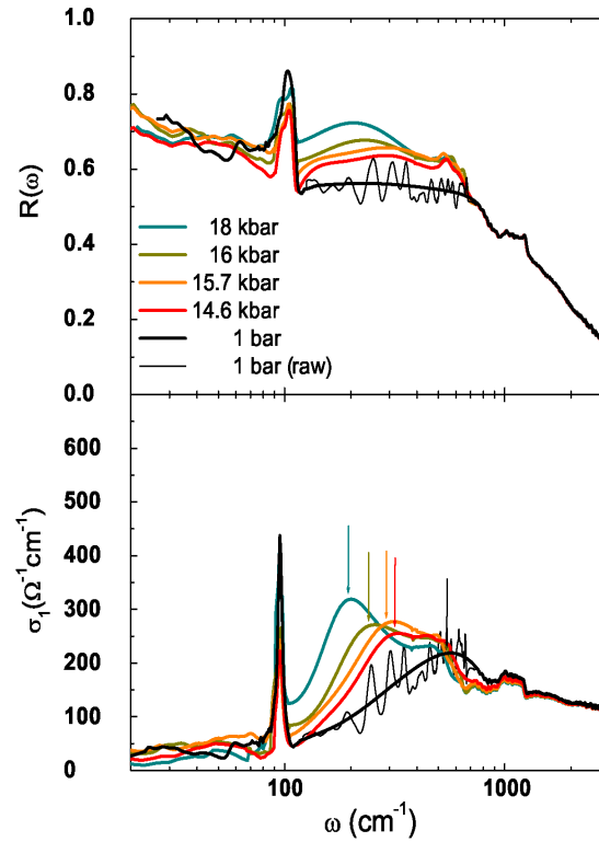
Figure 8.3: The reflectivity (upper panel) and conductivity (lower panel) spectra of \text{BaVS}_3 at a temperature lower than T_{MI} for selected pressures. The position of the gap at each pressure is indicated by the appropriately colored arrow.
