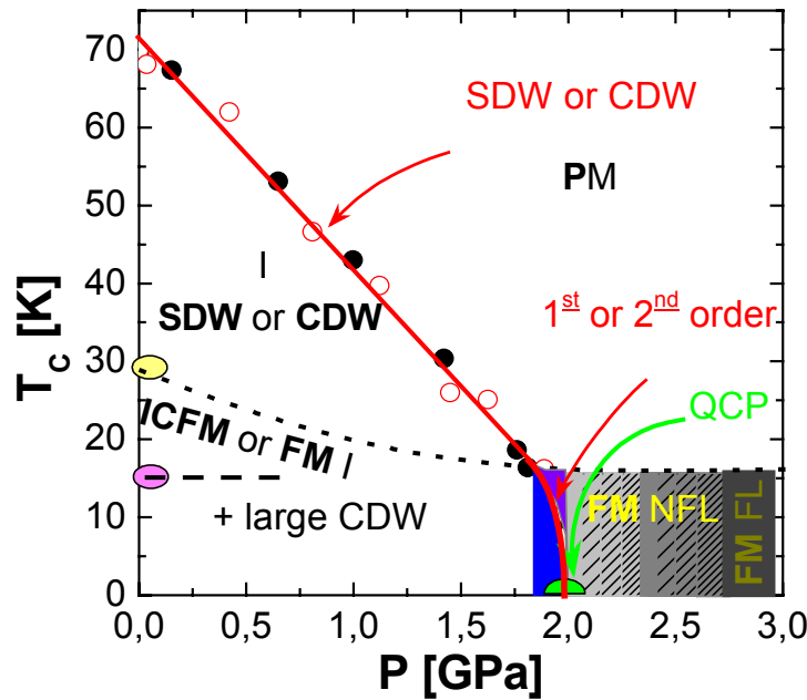
Figure 5.26: The proposed temperature-pressure phase diagram of BaVS 3 . Below p_{cr} all the phases or phase boundaries have double names related to the pure or impure samples, respectively. The MI phase boundary is marked by the red line. The temperature at which the (new) magnetic order starts to appear ( T_x \sim 30 K) is marked by the yellow spot while the temperature by which the magnetic order is completed ( \sim 15 K) is marked by a magenta spot. The probable extensions of these two points to high pressures are denoted by the dotted and dashed lines, respectively. The green spot symbolizes the QCP (at p_{cr} ), and the blue, the violet and the gray fields stand for the related fluctuation regions. The gray regions are related to crossover from NFL to FL marked by the power law temperature dependence of the resistivity. The increase of the value of n is represented by darker and darker gray color, the lightest gray symbolizing n = 1.5 and the darkest n = 2 .
