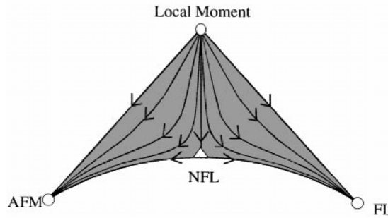
Figure 5.6: Schematic scaling diagram for the Kondo lattice competition of the two low temperature phases on the example of AFM - FL. QCP is marked by the white point at the end of the separatrix between two different types of trajectories. (Coleman, 1999)
