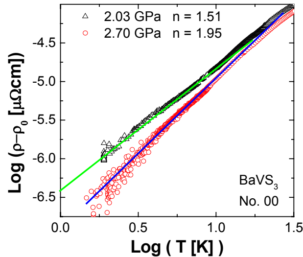
Figure 5.8: Logarithmic plot of the resistivity in BaVS 3 for a pressure close to the QCP (black points), and in the FL phase (red points).
