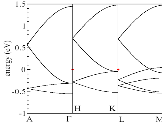
Figure 3.18: Electronic dispersion, for the three (six) band model, in the k_z direction for the same set of parameters as used to generate Fig. 3.17, except that the parameter describing the d_z^2 - e(t_{2g}) splitting is now set to be 3\Delta = 1 eV. The zero of energy is taken arbitrarily.
