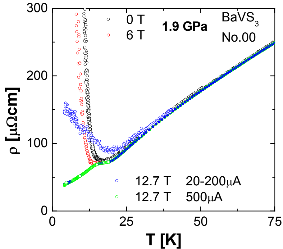
Figure 5.20: Resistivity as a function of temperature and current for three magnetic fields, at a pressure of 1.9 GPa. For the two lowest fields, no current dependence was observed. At 12.7 T electrical properties differ if the resistivity was measured keeping the DC current as low as possible (20 - 200 \mu A) or at higher current of 500 \mu A.
