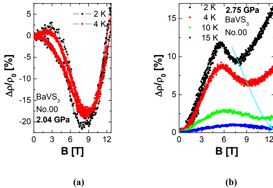
Figure 5.24: Isothermal magnetoresistance curve recorded at different temperatures and pressures. (a) The 2 and 4 K curves at 2.04 GPa. (b) Curves taken at 2.75 GPa for several temperatures. The cyan arrow indicates the position of the dip for various temperatures.
