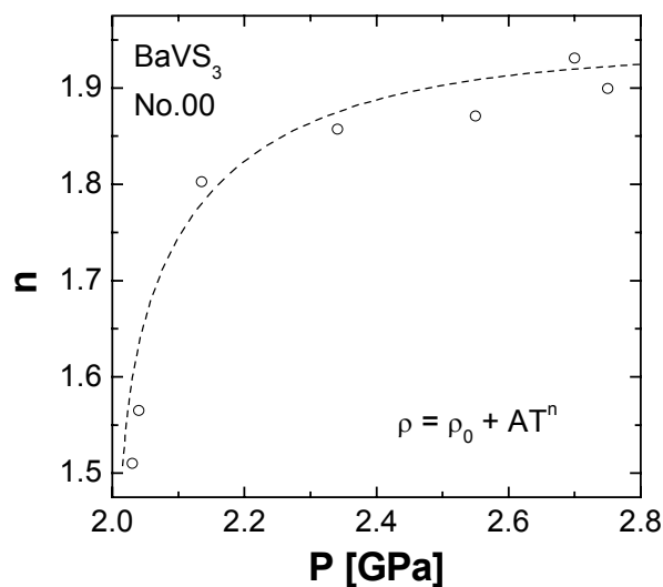
Figure 5.14: Pressure dependence of the resistivity exponent n . The dashed line is to guide the eye.
