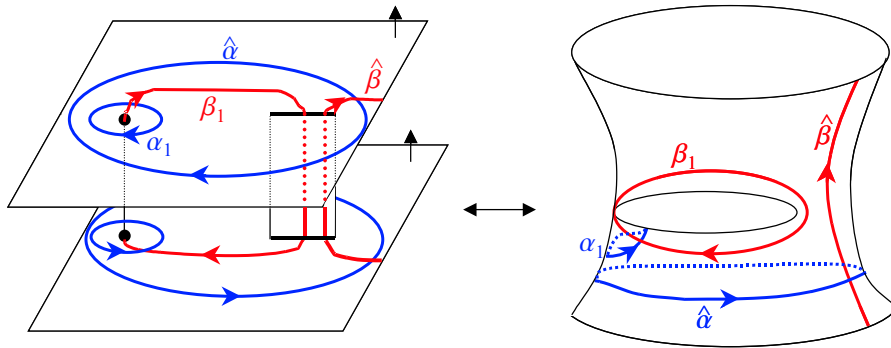
Figure 5.1: The Riemann surface for a cubic tree level potential, and f_0 such that one of the two cuts collapses to a point.
