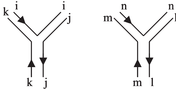
Figure 4.3: To calculate \langle (\text{tr } M^3)^2 \rangle one has to sum over all the possibilities to connect two trivalent vertices.
