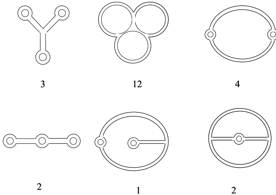
Figure 4.5: All possible planar diagrams containing four vertices, together with their symmetry factors |Aut(\Gamma)| .
