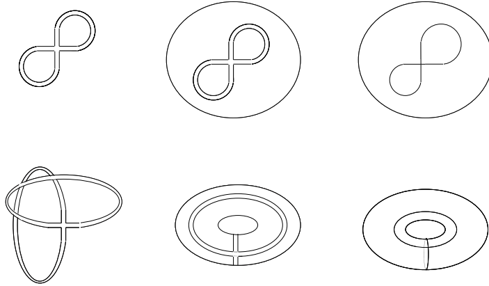
Figure 1.2: The appearance of a Riemann surface for two fatgraphs. The first graph can be drawn on a sphere and, after having shrunk the fatgraph to a standard graph, it can be understood as its triangulation with three faces, two edges and one vertex. The second graph, on the other hand, can be drawn on a torus. The corresponding triangulation has two edges, one vertex and only one face.
