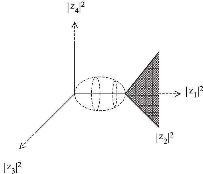
Figure 3.4: The part of \mathbb{R}_+^3 that is the base of the T^3 fibration of the resolved conifold is bounded by the surfaces |z_1|^2 = 0 , |z_3|^2 = 0 , |z_4|^2 = 0 and |z_2|^2 = 0 . If k of these equations are satisfied simultaneously, k of the S^1 s in T^3 shrinks to zero size. In particular, at |z_3|^2 = |z_4|^2 = 0 one has a single S^1 in the fibre that shrinks at |z_1|^2 = 0 and |z_1|^2 = t . The set of these S^1 form the \mathbb{P}^1 in C_{res} .
