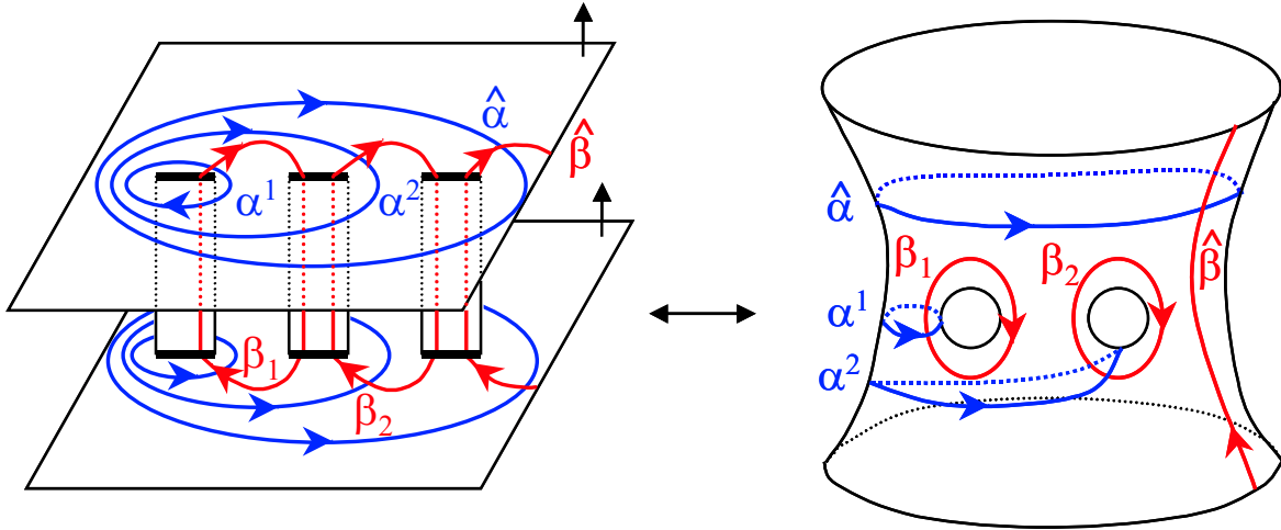
Figure 3.1: The hyperelliptic Riemann surface (3.1) can be understood as two complex sheets glued together along cuts running between a_i^- and a_i^+ . Here we indicate a symplectic set of cycles for \hat{g} = 2 . It consists of \hat{g} compact cycles \alpha^i , surrounding i of the cuts, and their compact duals \beta_i , running from cut i to i + 1 on the upper sheet and from cut i + 1 to cut i on the lower one. We also indicated the relative cycles \hat{\alpha} , \hat{\beta} , which together with \alpha^i, \beta_i form a basis of the relative homology group H_1(\Sigma, \{Q, Q'\}) . Note that the orientation of the two planes on the left-hand side is chosen such that both normal vectors point to the top. This is why the orientation of the \alpha -cycles is different on the two planes. To go from the representation of the Riemann surface on the left to the one on the right one has to flip the upper plane.
