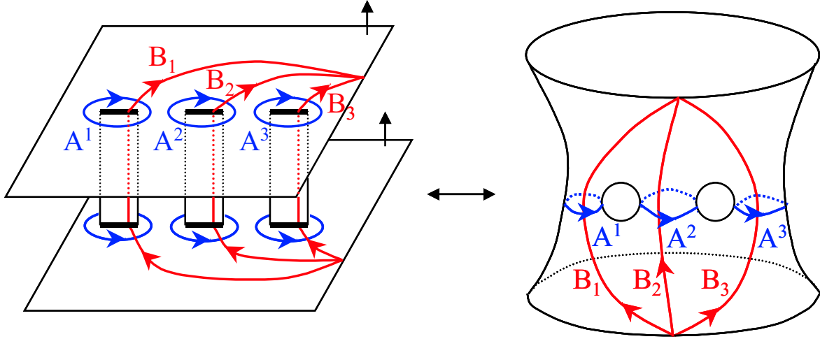
Figure 3.2: Another choice of basis for H_1(\Sigma, \{Q, Q'\}) containing compact A-cycles and non-compact B-cycles.
