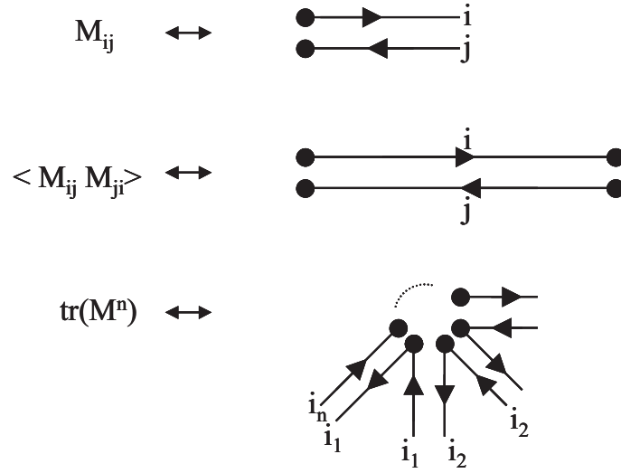
Figure 4.2: The Feynman diagrammatic representation of the matrix M_{ij} , the propagator \langle M_{ij} M_{ji} \rangle_G and an n -valent vertex \text{tr}(M^n) .
