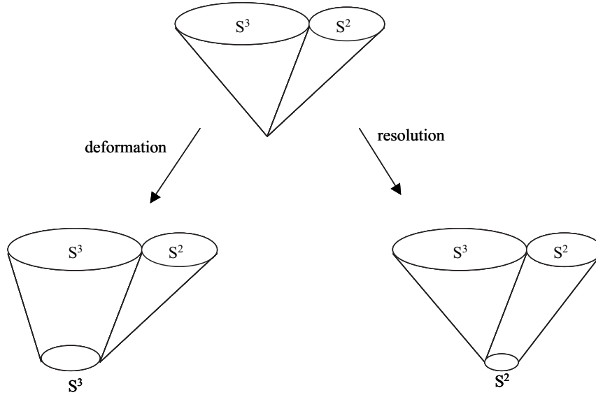
Figure 3.3: The conifold is a cone over S^3 \times S^2 with a conical singularity at its tip that can be smoothed out by a deformation or a small resolution.
