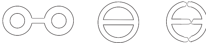
Figure 4.4: From two three-valent vertices one can draw three Feynman diagrams, two of which can be drawn on the sphere, whereas the last one is “nonplanar”.
