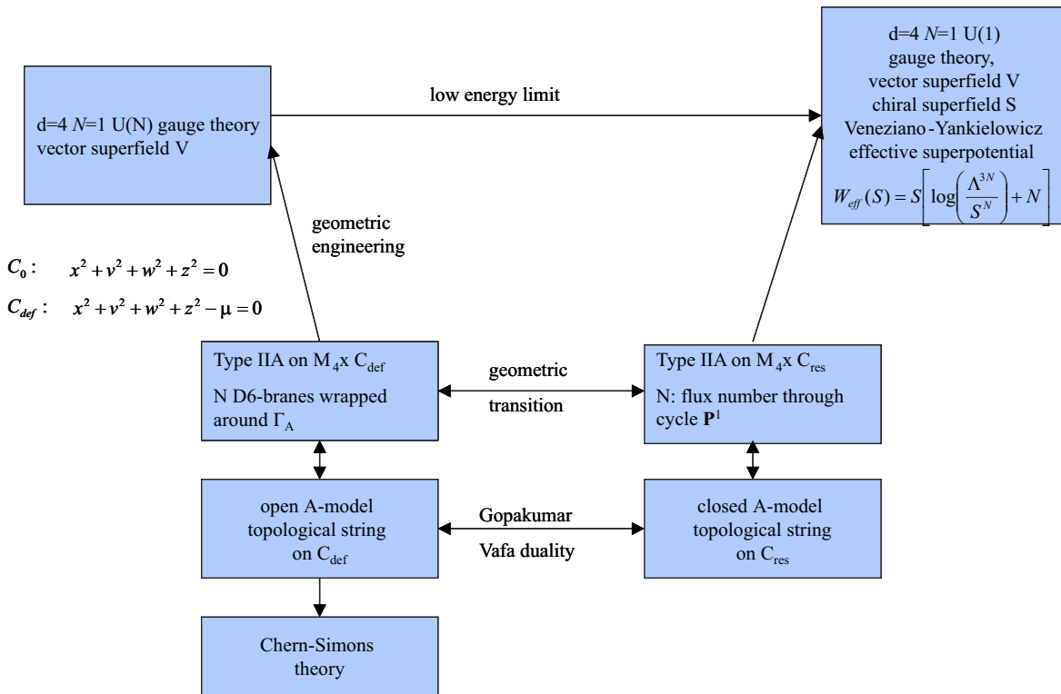
Figure 1.4: A sketch of the relation of supersymmetric Yang-Mills theory with Type IIA string theory on the conifold and with Chern-Simons theory.
