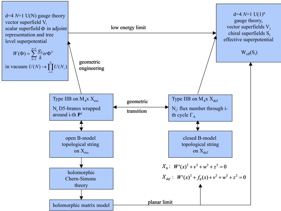
Figure 1.3: A sketch of the relation of supersymmetric Yang-Mills theory with Type IIB string theory on non-compact Calabi-Yau manifolds and with the holomorphic matrix model.
