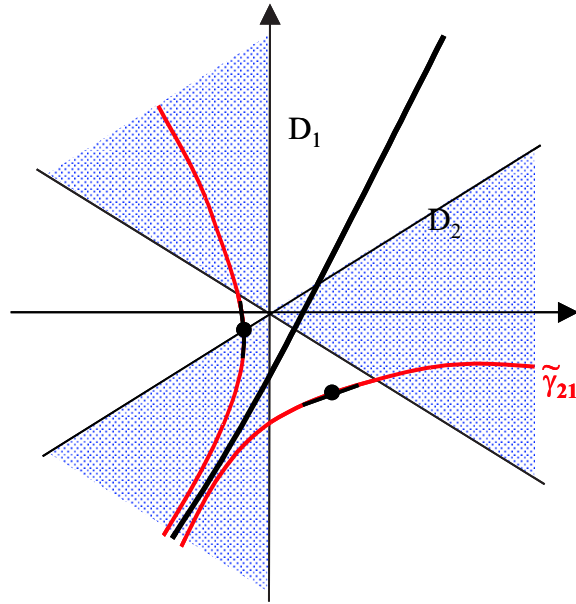
Figure 4.6: For the cubic potential of Fig. 4.1 we show the choice of the domains D_1 and D_2 (to the left and right of the bold line) and of the path \tilde{\gamma}_{21} with respect to the two critical points, as well as the cuts that form around these points.
