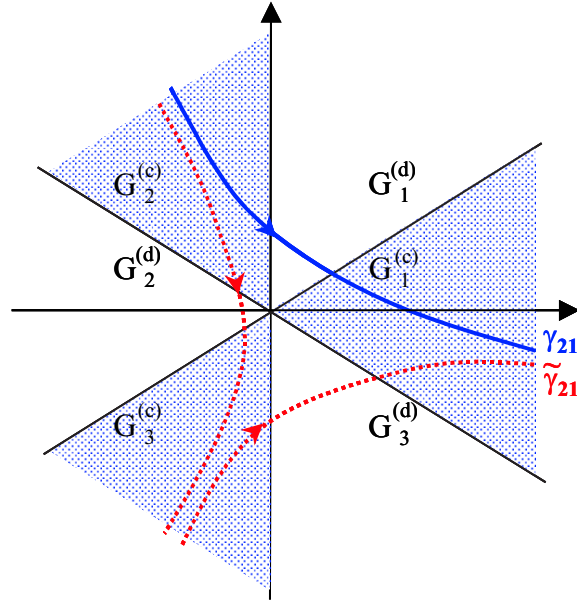
Figure 4.1: Example of convergence and divergence domains for n = 2 and a possible choice of \gamma_{21} . Because of holomorphicity the path can be deformed without changing the partition function, for instance one could use the path \tilde{\gamma}_{21} instead.
