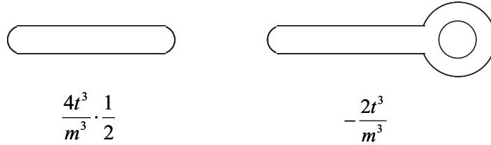
Figure 5.2: The linear term in W leads to tadpoles in the Feynman diagrams, each tadpole coming with \frac{2tg}{mg_s} , which contains a factor of g . At order g^2 only two diagrams contribute.
