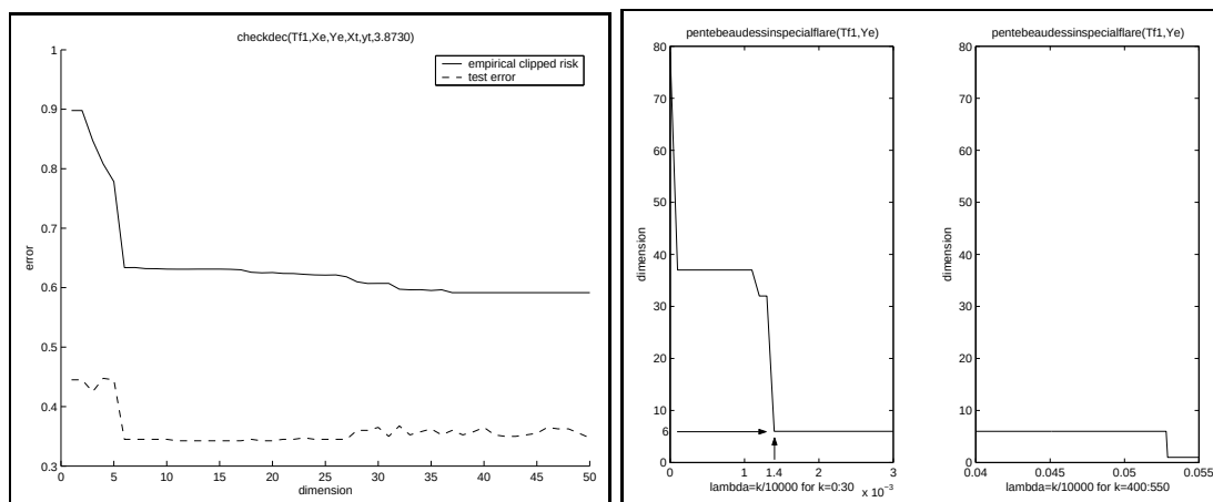
Figure 6.3: Left: The straight line is the empirical risk for the clipped soft loss function P_n \gamma(\tilde{f}_D) and the dashed line is the test error. Both on 'flare-solar' Right: Selected dimension \hat{D} versus \lambda using (6.21).
