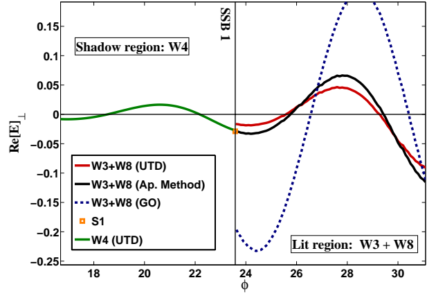
(b) Section SSB1
