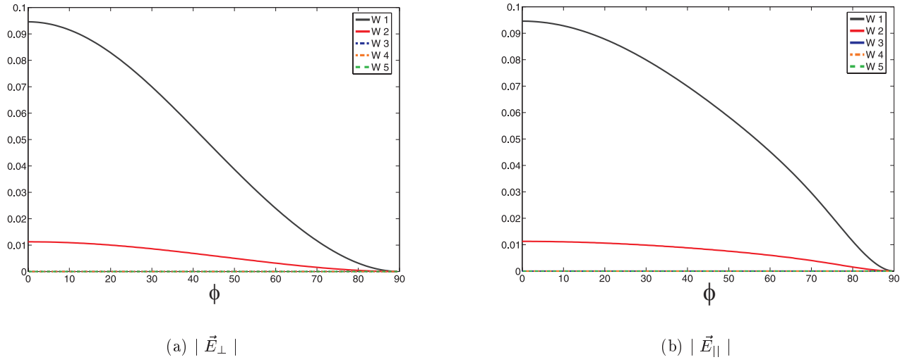
Figure 5.9: Ray contributions \vec{E}_\perp^0 = 1 , \vec{E}_\parallel^0 = 1 , f = 500MHz , \epsilon_2 = 9.6 - i , d = 0.5m
