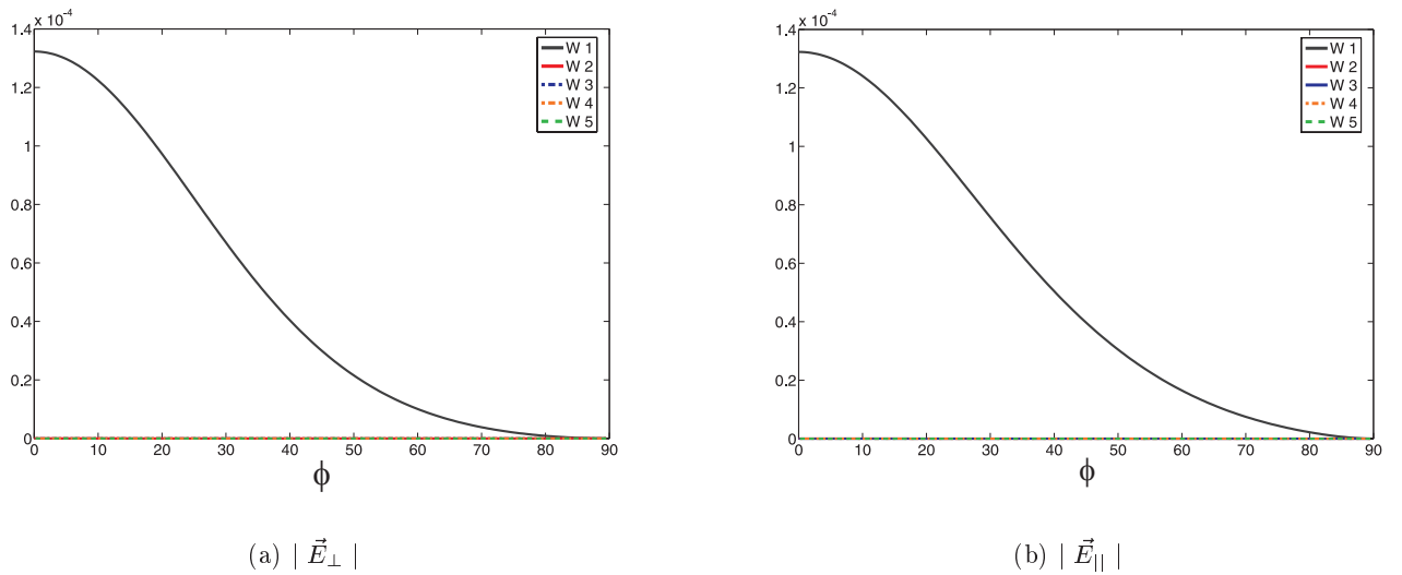
Figure 5.10: Ray contributions \vec{E}_\perp^0 = 1 , \vec{E}_\parallel^0 = 1 , f = 500MHz , \epsilon_2 = 9.6 - 5i , d = 0.5m
