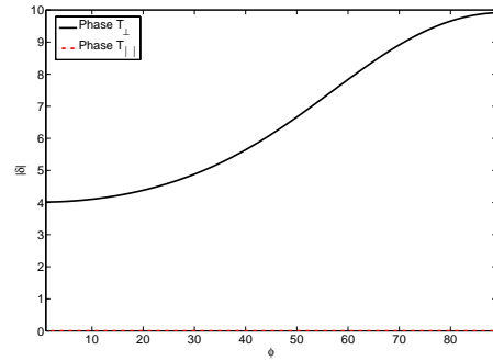
Figure 5.16: \epsilon_2 = 9.6 - 8i
