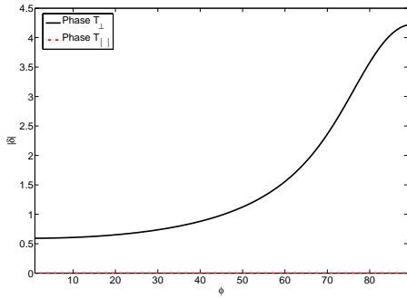
Figure 5.15: \epsilon_2 = 9.6 - i
