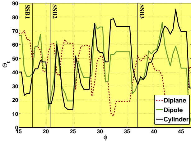
Figure 6.7: EMSL h = 10.0\text{cm} , f = 6.7\text{GHz}
