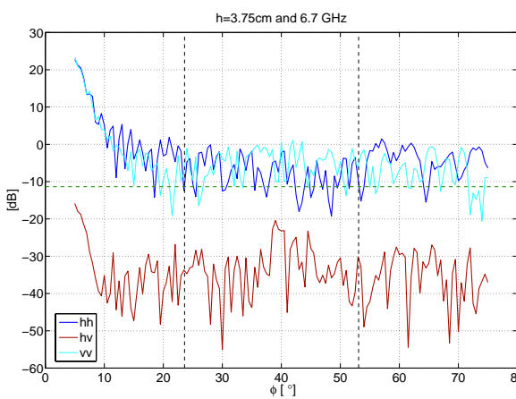
Figure 4.5: RCS of single field components h_1 = 3.75\text{cm}
