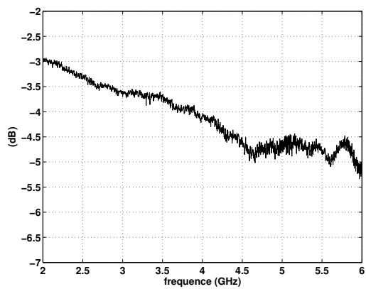
(c) S21
