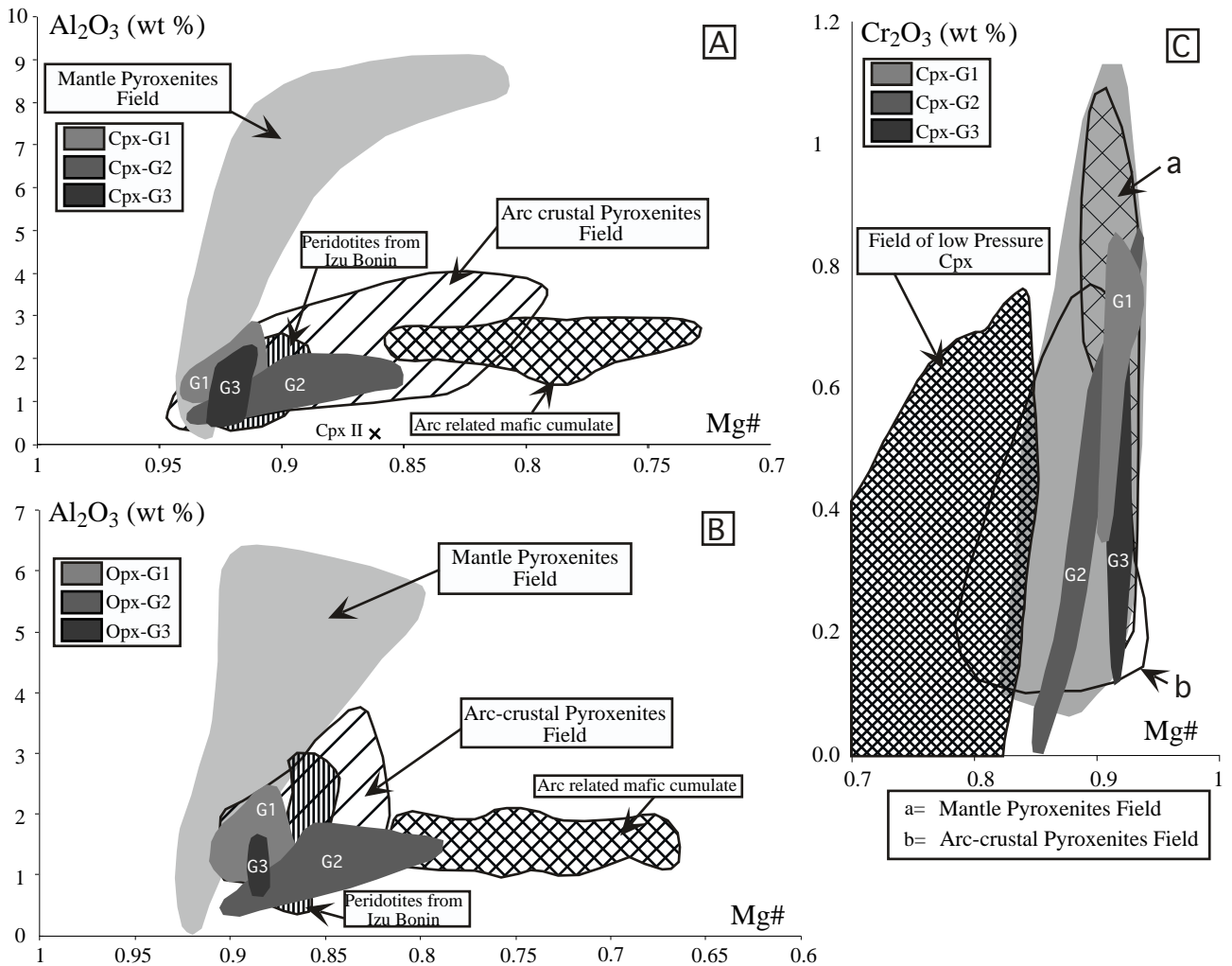
Fig. 3-21: A) Plots of \text{Al}_2\text{O}_3 versus Mg# for the clinopyroxene (A) and orthopyroxene (B) and plot of \text{Cr}_2\text{O}_3 versus Mg# (C) for the clinopyroxene. References are from arc-related peridotites (Parkinson and Pearce, 1998), mantle pyroxenites (Kornprobst, 1969; Irving, 1974, 1980; Frey et al., 1978; Sinigoi et al., 1980; Bodinier et al., 1987, 1988; Seyler et al., 1989, 1993; Griffin et al., 1988; Piccardo et al., 1988, Shervais, 1990; Pearson et al., 1993; Rivalenti et al., 1995; Vaselli et al., 1995; Kumar et al., 1996; Wilkinson and Stolz, 1997; Garrido et al., 1999; Zanetti et al., 1999; McInnes et al., 2001) and arc-related igneous pyroxenites (Findlay, 1969; James, 1971; Jan and Howie, 1981; Quick, 1981; Snoke et al., 1981; DeBari and Coleman, 1989; Girardeau and Ibaruchi, 1991; Kausar, 1998; Smith et al., 1999; Parlak et al., 2002; Santos et al., 2002; Spandler et al., 2003; Worden, 2002).
