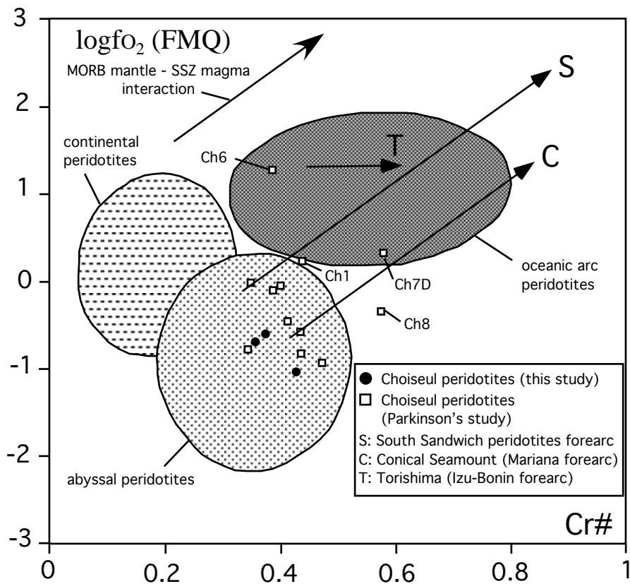
Fig. 2-12: Plot of \log f_{\text{O}_2} (FMQ) against Cr# of spinel for the Choiseul peridotites. Fields for abyssal peridotites, arc peridotites and continental peridotites are after Pearce et al., 2000. Reference is made to peridotite data from Conical Seamount (C) in Mariana Forearc and Torishima Forearc Seamount (T) in the Izu-Bonin forearc (Parkinson et al., 1998).
