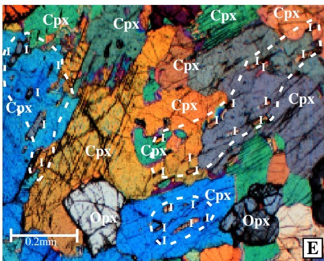
Fig. 3-4: Textural characteristics of the pyroxenites from San Jorge and Isabel.
