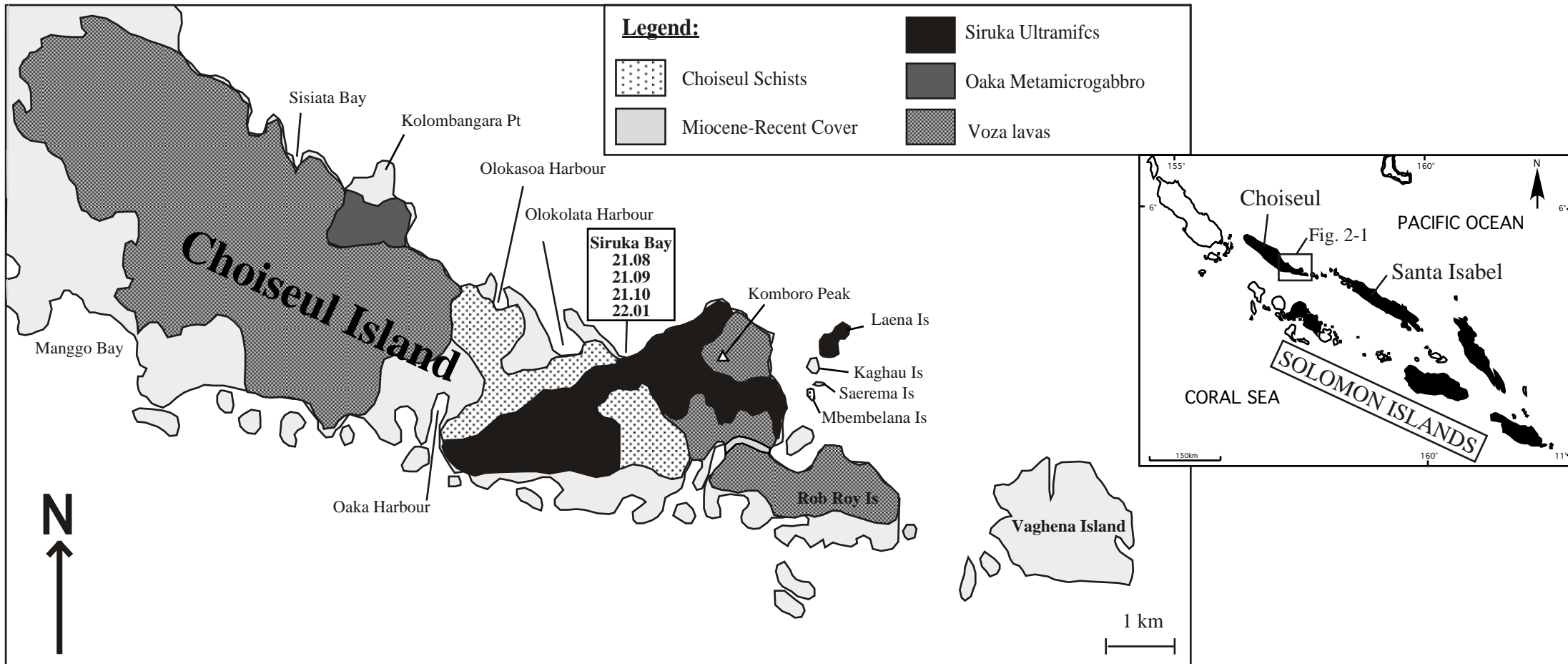
Fig. 2-1: Simplified geological map of southern part of Choiseul (after I. J. Parkinson, pers., comm.)
