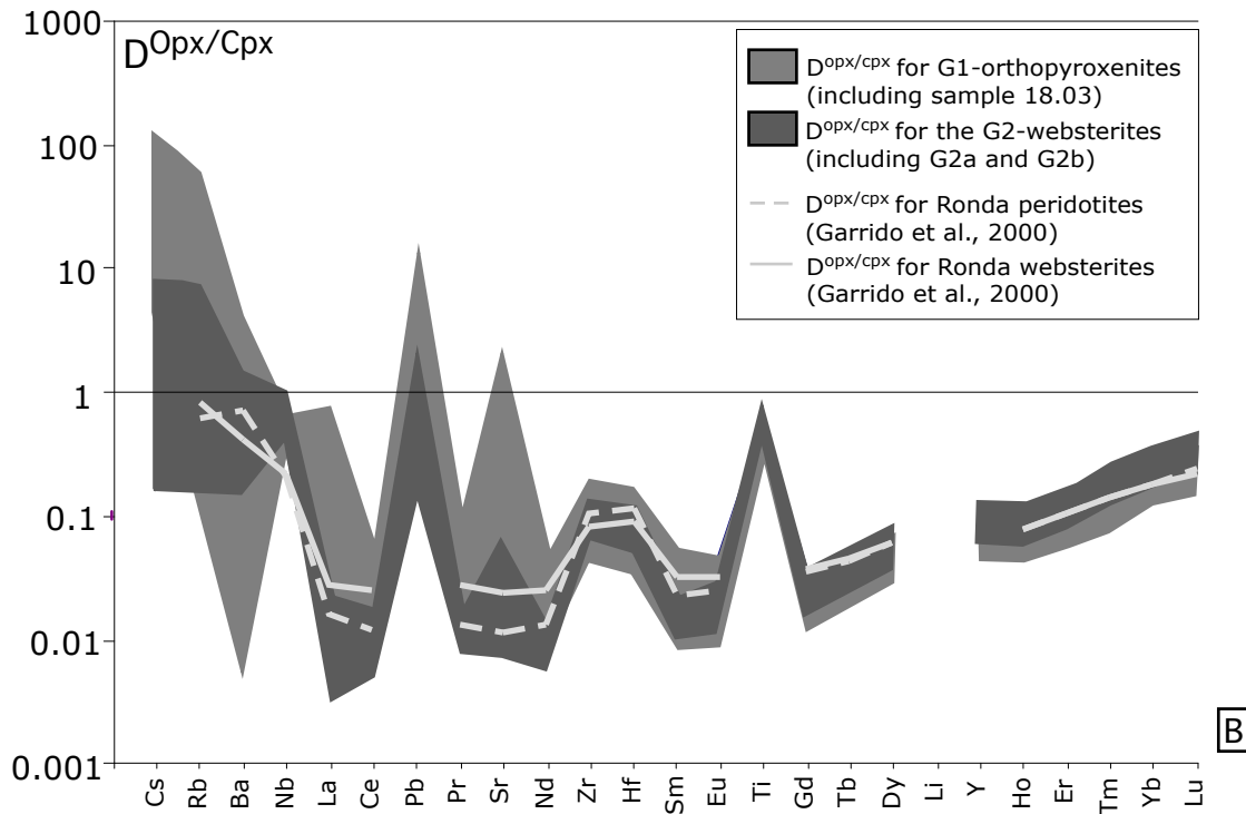
Fig. 4-15: Average D^{Opx/cpx} for REE (A) and extended trace elements (B) of the G1-orthopyroxenites and the G2-websterites.
