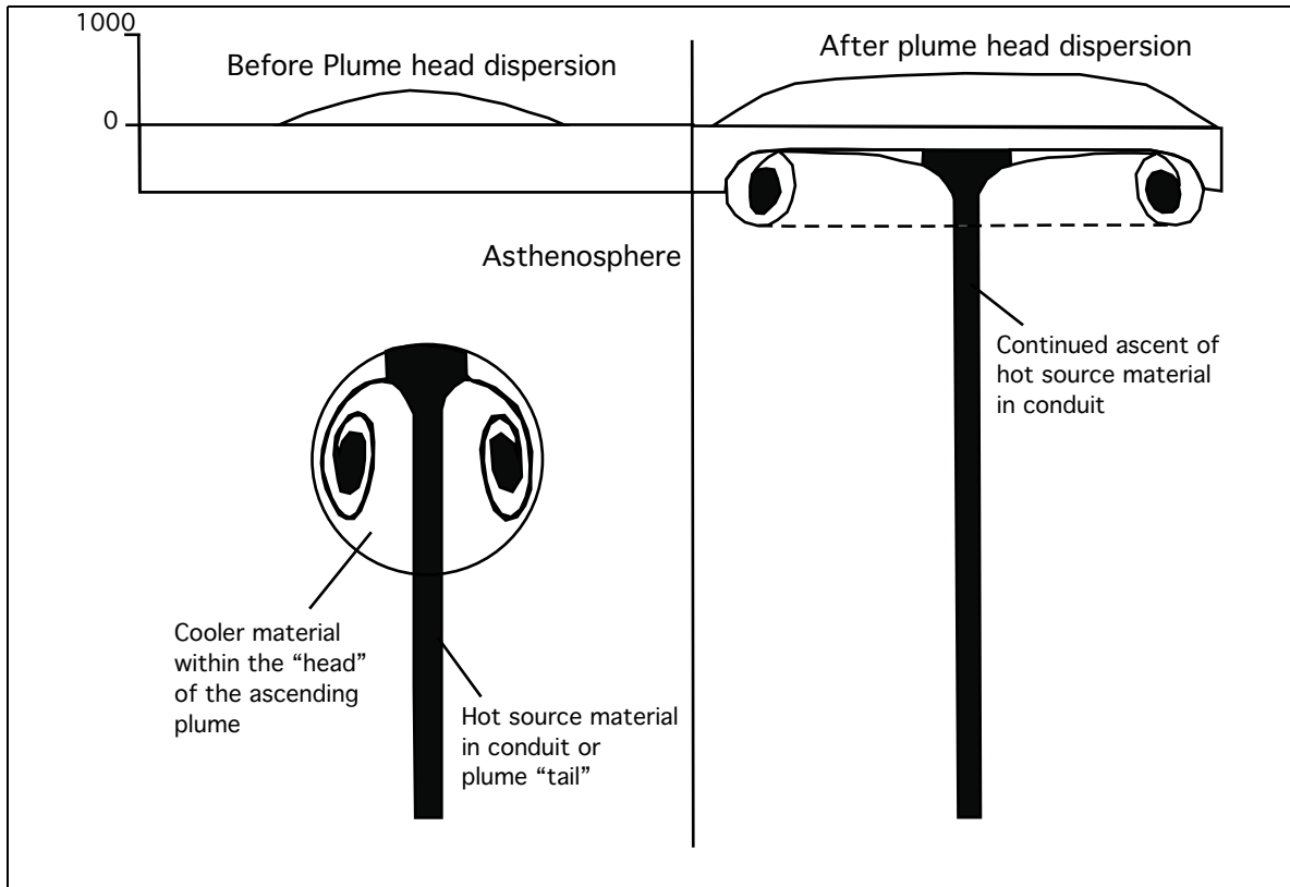
Fig. 1-5: Model for LIP generation and emplacement (after Coffin and Eldholm, 1994).
