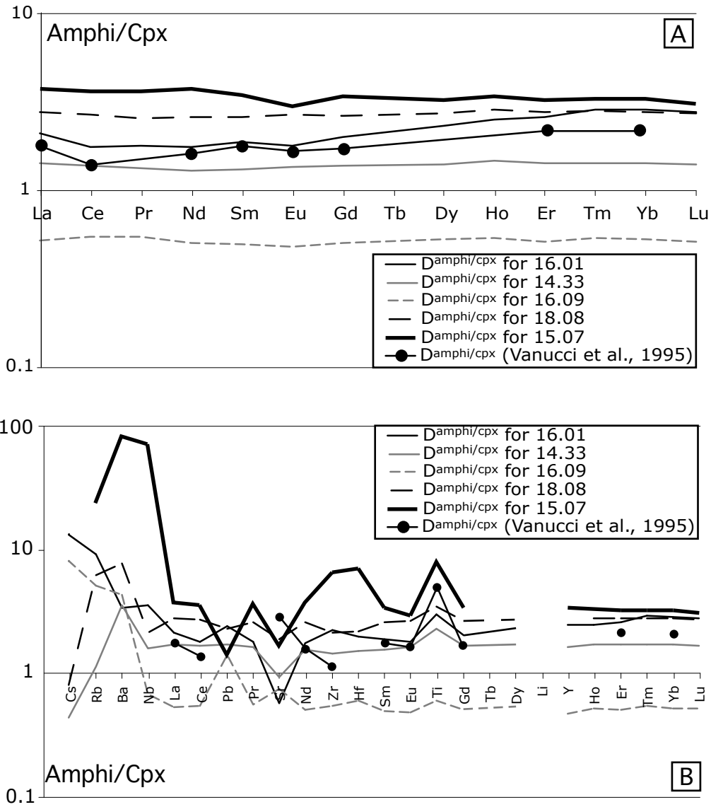
Fig. 4-17: Average D_{amphi/cpx} for REE (A) and extended trace elements (B) of some of the pyroxenites.
