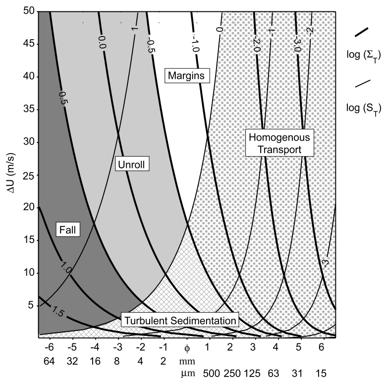
Figure 2.1 The interaction of 1000 kg/m 3 particles of various sizes (x-axis) with eddies of rotation speed \Delta U (y-axis) and a diameter \delta=10 m. Thin curves are Stokes numbers \log(S_T) and thick curves are Stability factors \log(\Sigma_T) . See text for the significance of Fall , Unroll , Margins , Homogenous Transport , and Turbulent Sedimentation zones.
