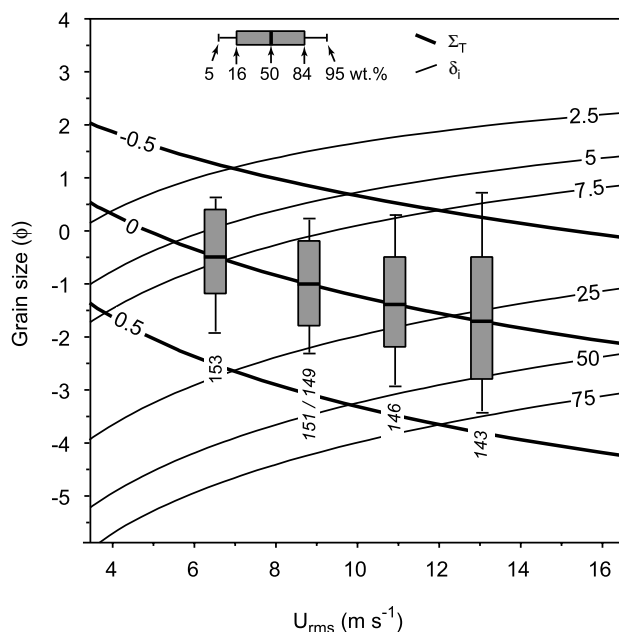
Figure 3.23 Example of backward modeling of field data using a U_{rms} vs. grain size plot. Samples are from the section IIIa (see text). Thick lines are \log(\Sigma_T) , thin lines are eddy maximum size \delta_i , and boxes represent grain size distributions. Variables used are \mu=1.5 \times 10^{-5} Pa s, \nu=3 \times 10^{-5} m 2 s -1 (air at 300 °C), and \rho_p = 1150 kg m -3 .
