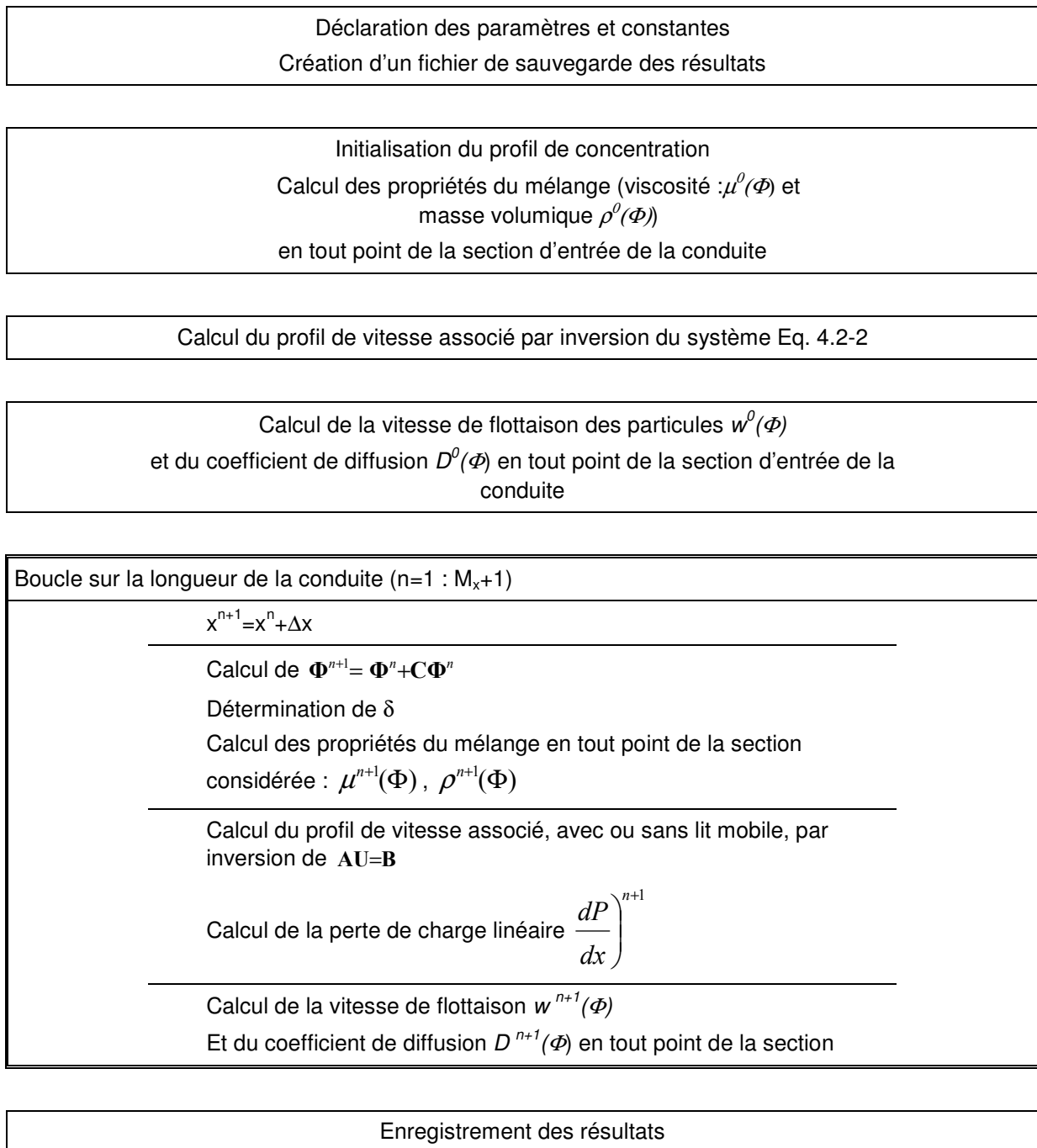
Figure 4.2-5 : Structure du programme principal
