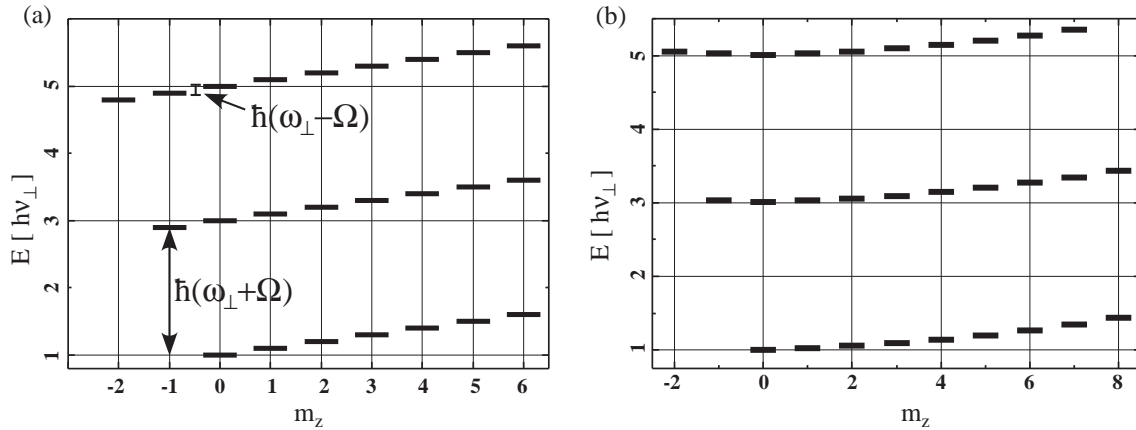
Figure 9.1: Single particle states of fast rotating condensates. a) Landau levels in a harmonic trap for \Omega = 0.9 \omega_{\perp} . (b) In a quadratic+quartic trap the structure of the Landau levels is modified as compared to the purely harmonic case. In this graph \Omega = \omega_{\perp} , and the strength of the quartic term is larger by a factor 10 as compared to the experimental case, to make the quadratic variation more visible.
