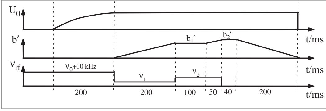
Figure 4.11: Experimental routine for the separation of a single or several 2D condensates. The gradient is ramped to an intermediate value b'_1 . During this ramp the “lower” part of the cigar is driven through the rf knife at the value \nu_1 . The rf frequency is then set to \nu_2 = \nu_1 + \Delta , before the gradient is ramped to its final value b'_2 > b'_1 . This ramp eliminates the sites in the “upper” part of the cigar. This routine spares all sites within the frequency gap \Delta .
