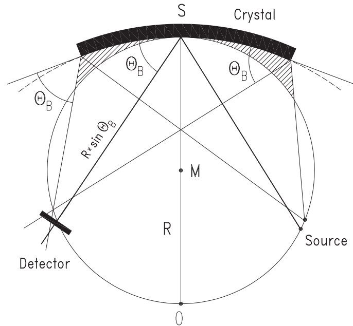
Figure 3.12 – The Johann setup for Bragg spectroscopy. The crystal bending radius R = SO is the diameter of the Rowland circle (with the center at M ) on which the focusing condition R \sin \Theta_B is fulfilled. X-rays reflected from the lateral sides of the crystal are focalized in a different point on the Rowland circle than the X-rays reflected from the central side of the crystal. This effect causes a shift of the line centroid to smaller values of Bragg angle (higher energies).
