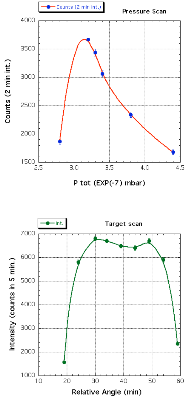
Figure 5.11 – Pressure scan (top) and target scan (bottom) of the ECR plasma with sulphur, using quartz ( 10\bar{1} ) crystal. The target scan enables to study the spatial distribution of ionized ions in the plasma. The total pressure of the gas in the source is a critical parameter and the optimal condition comes from a compromise between ionization and electron recapture probability.
