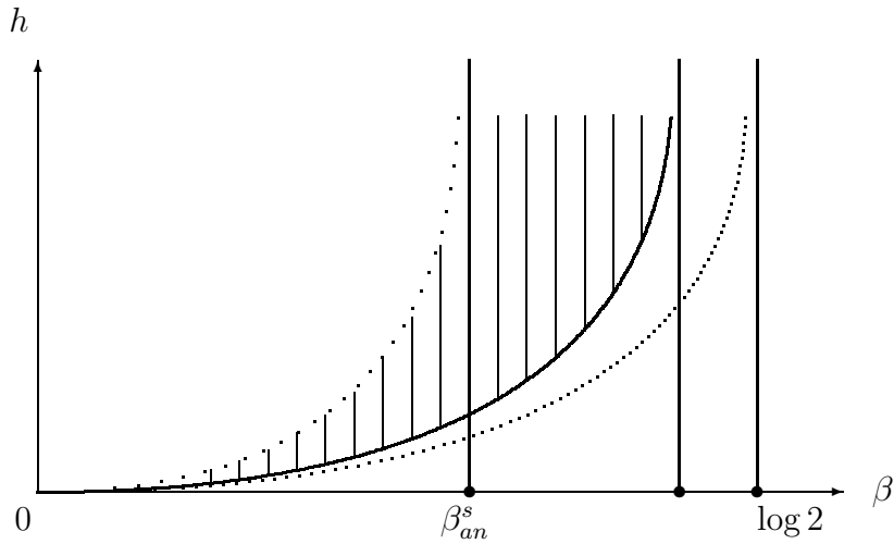
Fig. 1: ..... h_c^{an,s}(\beta) ————— m^s(\beta) possible location of h_c^s(\beta) ..... h_c^0(\beta)
